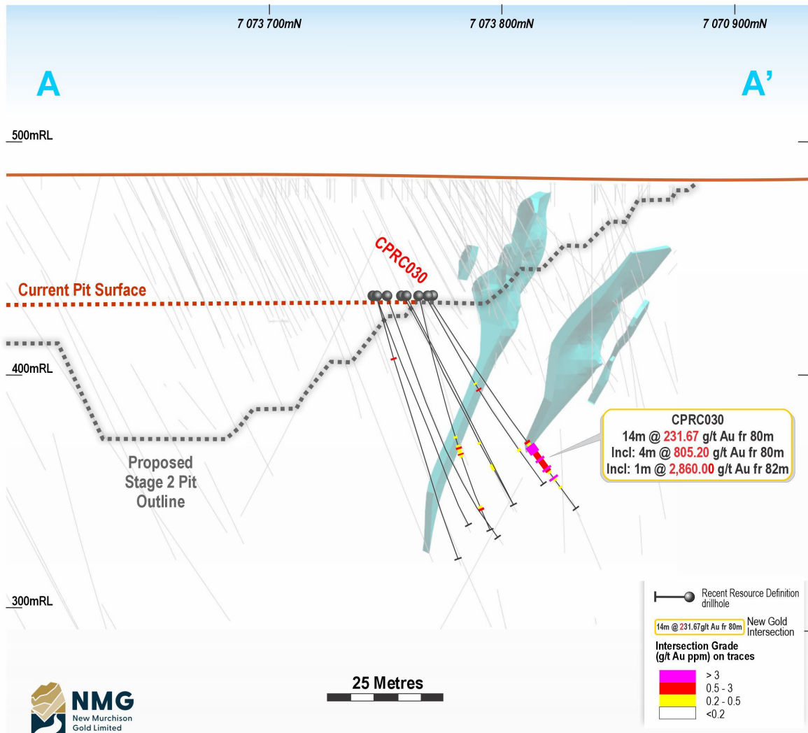
Figure 2: Cross-section A-A' (looking ENE, ±25m) through CPRC030 showing current MRE wireframes (blue solids) and grade on traces.
