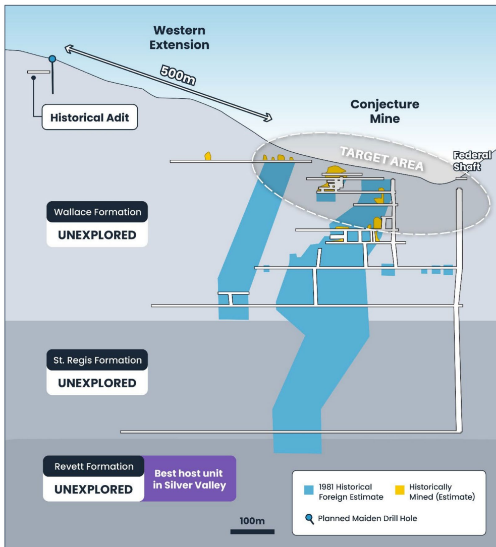
Figure 5: Conjecture Mine schematic long section (looking north-west) showing inferred geological boundaries, historically mined areas, the 1981 historical foreign estimate and the planned trace of the first drill hole
