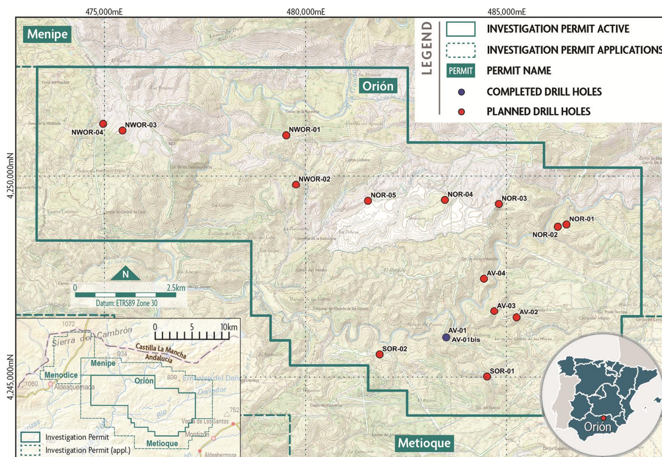
Figure 2 – Map showing location of planned and completed drill holes at Orión EU Critical Minerals Project.
