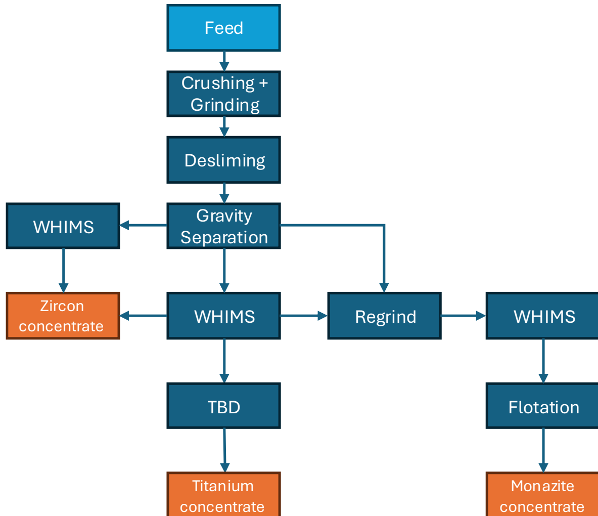
Figure 2 – Preliminary flowsheet schematic for Orión Project.
