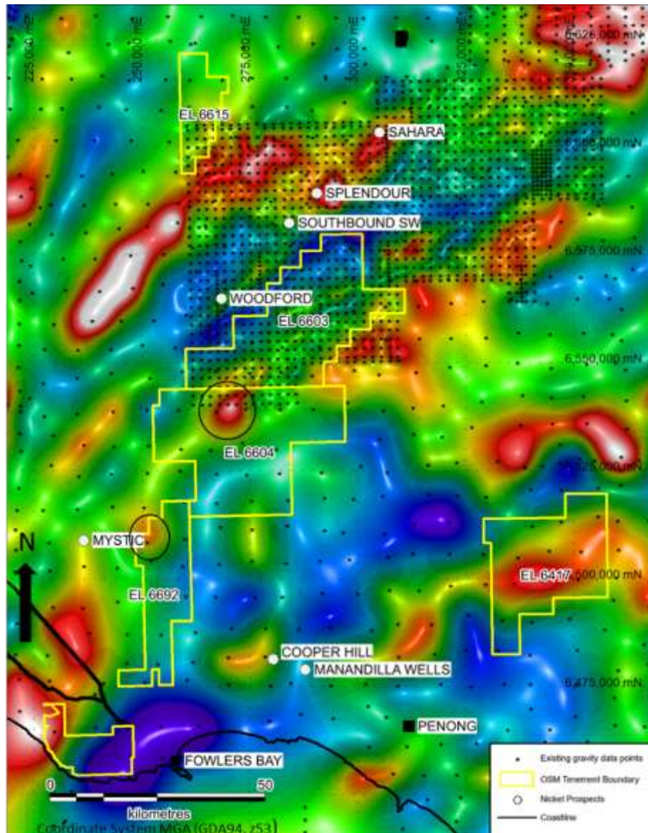
Figure 15: Residual Gravity image showing gravity data station density (black stars) and local Nickel Prospects. Priority targets areas are circled.
