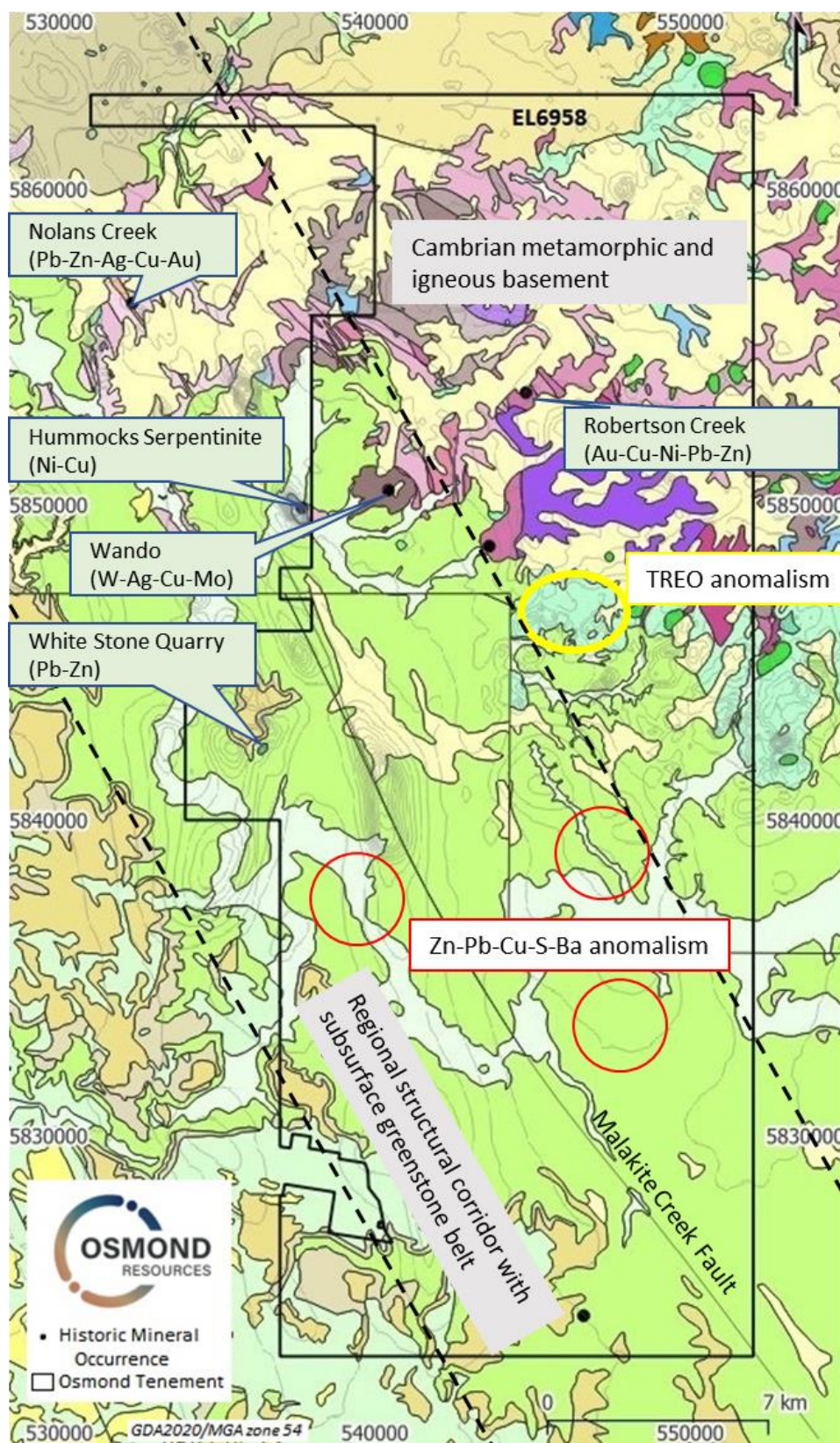
Figure 2: Sandford geology with historical mineral occurrences, soil sample anomalism (Base metals red, TREO yellow) and total magnetic intensity contours (grey)
