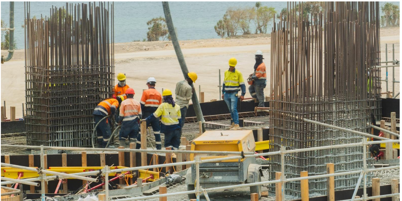
Image: PNG construction crew placing concrete on the Kiln 1 raised support deck, September 2026
