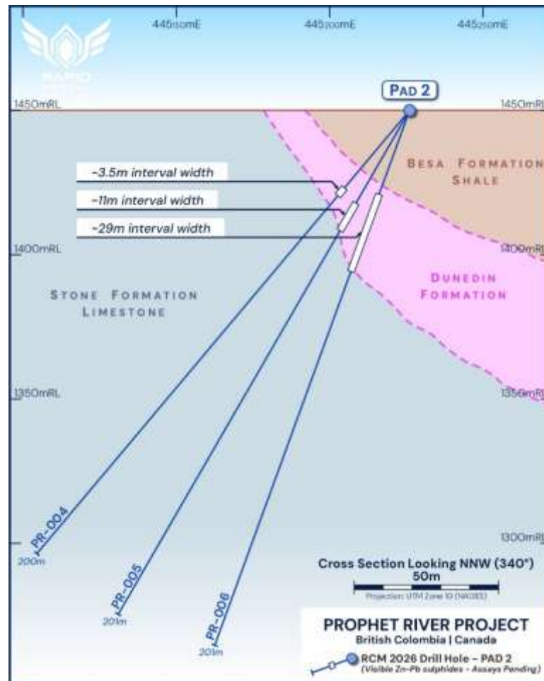
Figure 1: Cross-section through Pad 2 (looking 340°) showing the mineralised interval at the Dunedin/Stone Formation contact thickening with depth. Interval lengths from visual logging; true widths not yet known; assays pending.
