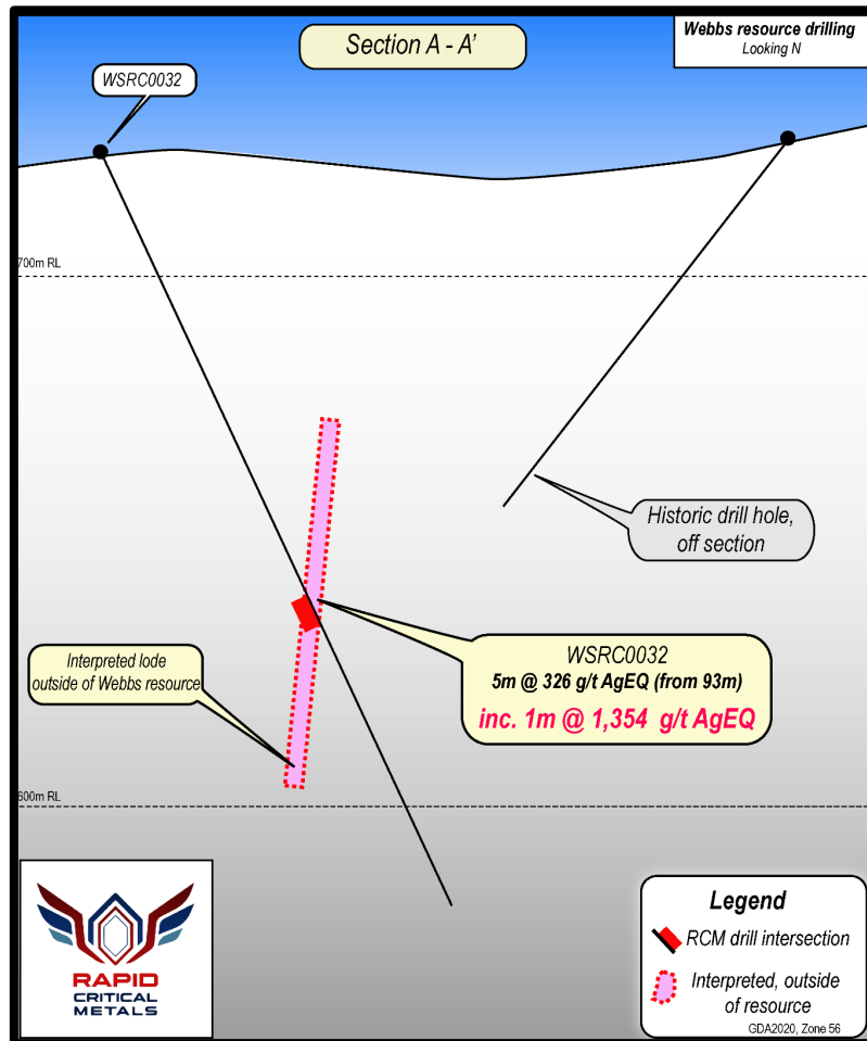
Figure 3: Section A–A’ on the plan (Figure 1): WSRC0032 – 5m at 326 g/t AgEQ from 93m, including 1m at 1,354 g/t AgEQ from 96m, in an interpreted lode outside the Webbs resource, 117m north of the resource outline. Historic drill hole shown off section. E–W section on approximately 6,752,990mN. True width is approximately 60% of down hole width.
