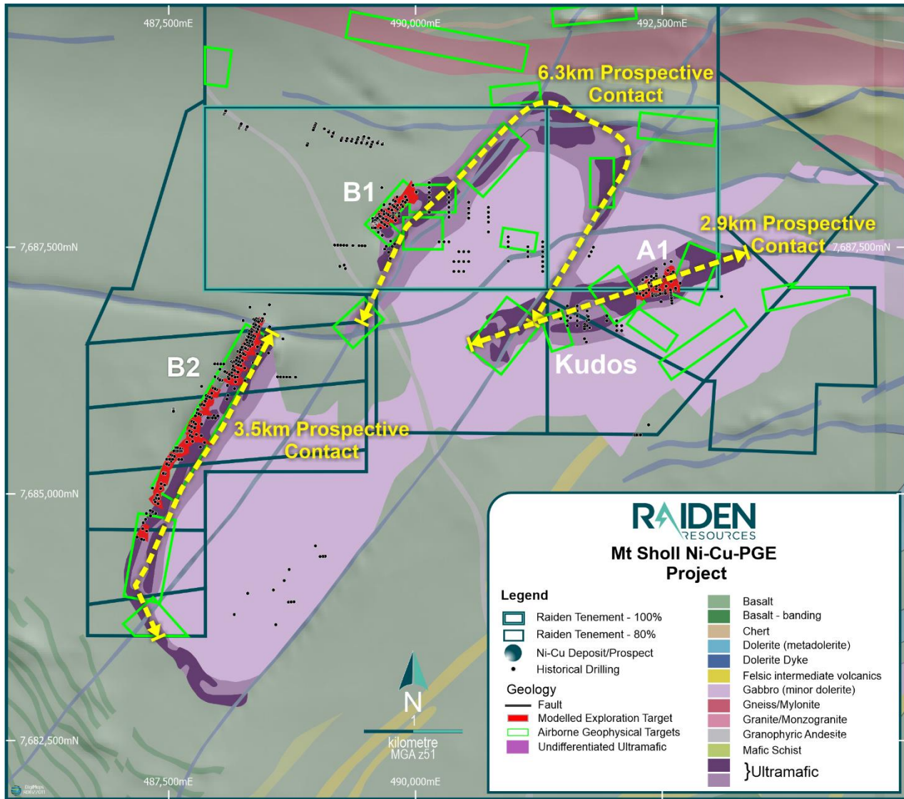
Figure 6: Mt Sholl Project area with Prospective Contact zones, drill hole locations over interpreted geology, JORC Exploration target 2 (red) and EM targets (green).
