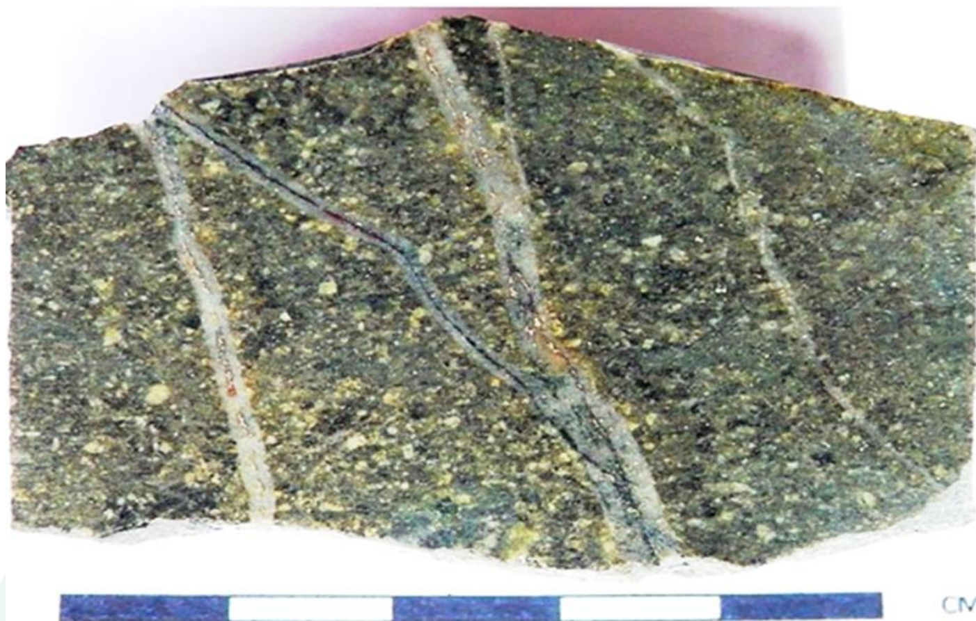
Figure 5 - Quartz-diorite porphyry, cut by banded quartz-sulphide-magnetite veins at surface
