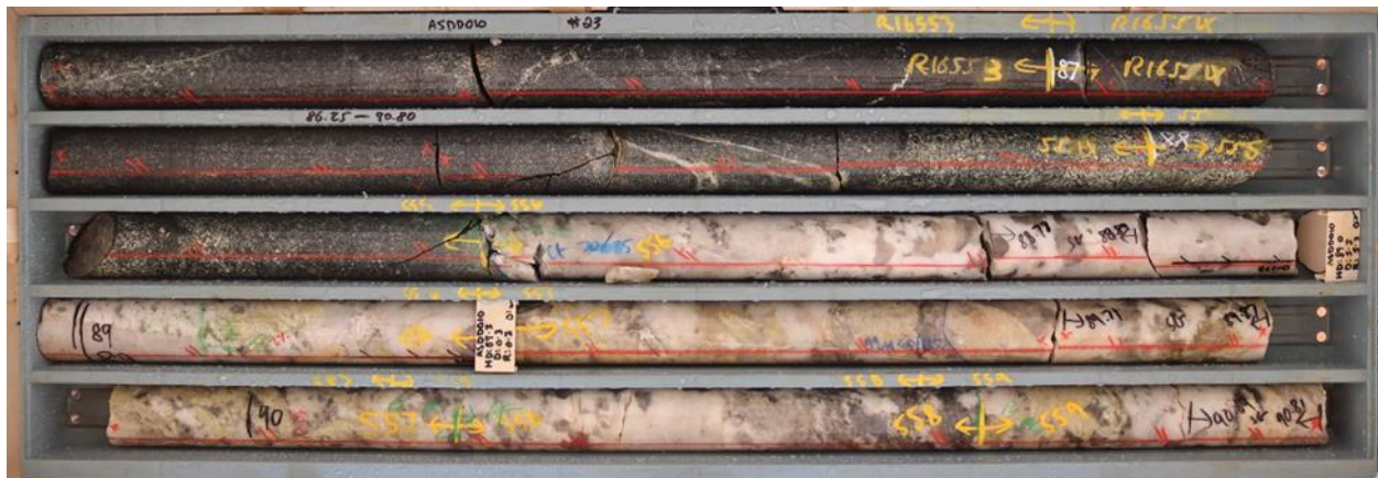
Figure 5: Drill core from ASDDO10 (high grade section - 90.56m to 90.96m interval - 2.1% Li 2 O)
