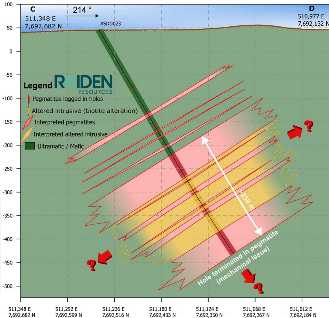
Figure 3: Interpreted cross-section of drill hole ASDD023 B
