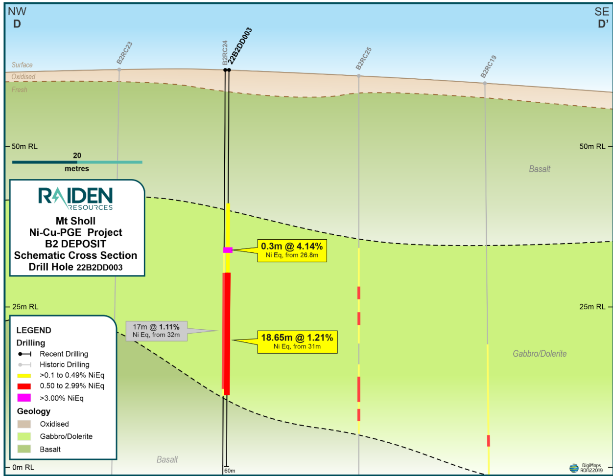
Figure 7: Section D-D' with recent hole 22B2DD003 and historical intercepts.
