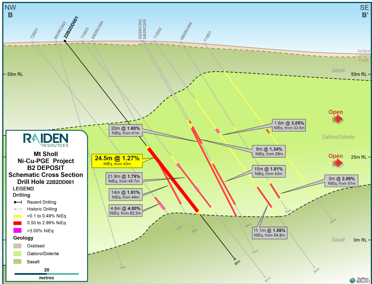
Figure 4: Section B-B' with recent hole 22B2DD001 and historical intercepts.
