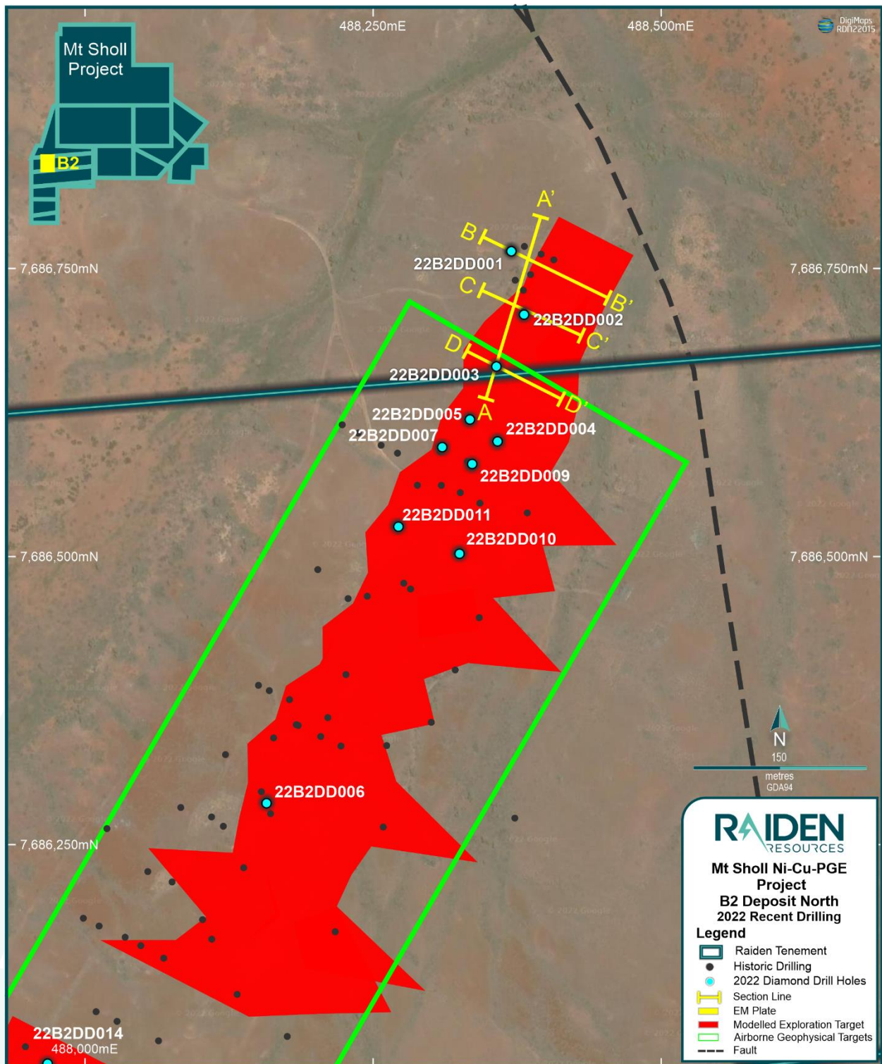
Figure 9: Mt Sholl B2 Deposit area with drill locations and section lines over JORC Exploration target. 2
