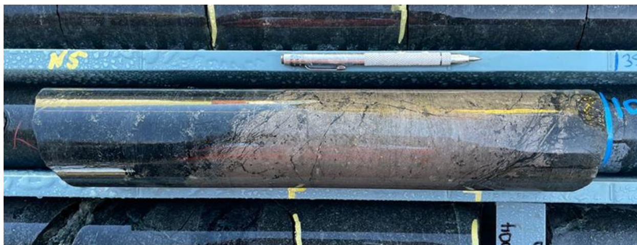
Figure 8: 22B2DD004 (25.1-25.6 metres – HQ core 61.1mm diameter) 0.5m @ 2.30% Ni Eq Strongly mineralised pyroxenite with fine-grained massive to semi-massive pyrrhotite with coarse minerals of pentlandite within a 47-metre zone of sulphide mineralisation.
