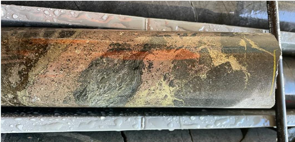
Figure 1: 22B2DD003 (26.8 -27.1 metre interval – NQ core 47.6mm diameter). 0.3m @ 4.14% Ni Eq Strongly mineralised dolerite with fine-grained pyrrhotite, chalcopyrite and coarse minerals of pentlandite. Mineralisation is semi-massive and interstitial.
