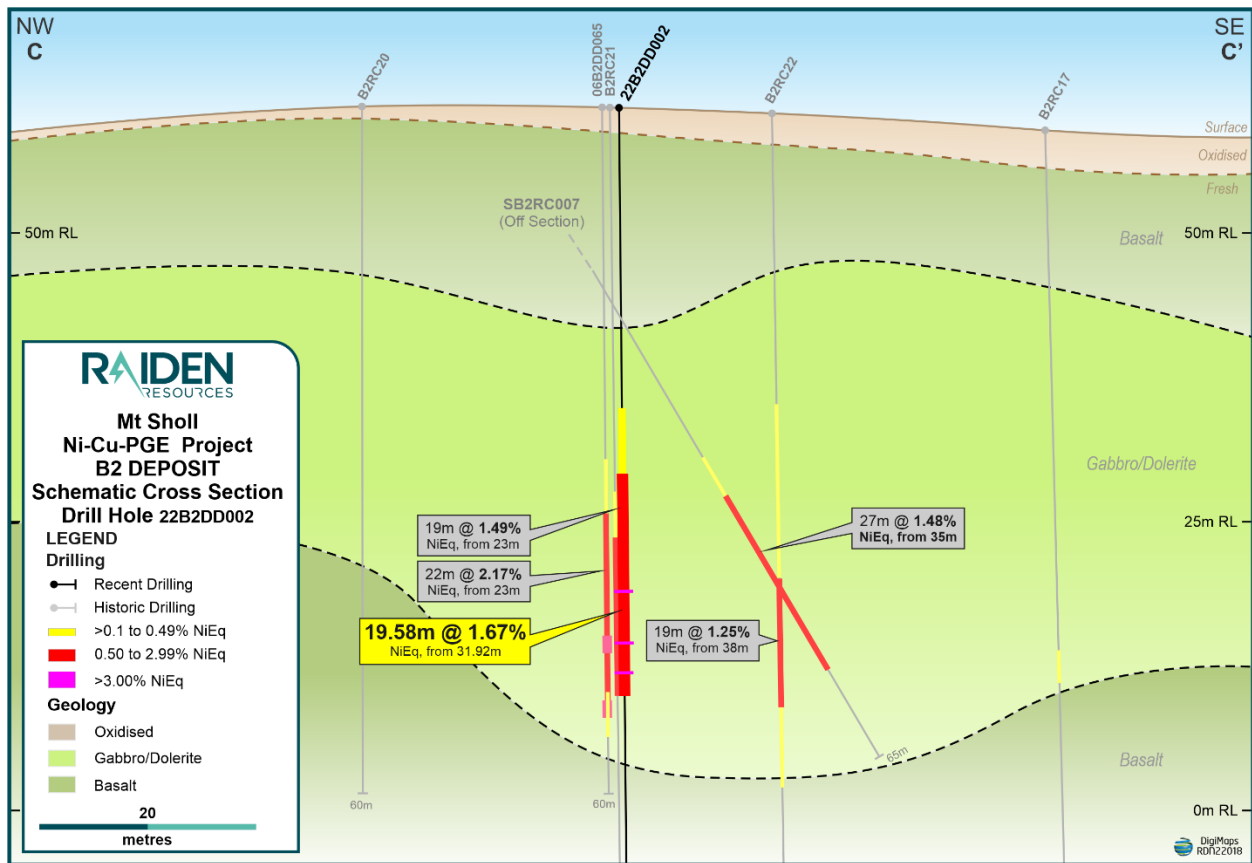
Figure 5: Section C-C' with recent hole 22B2DD002 and historical intercepts.
