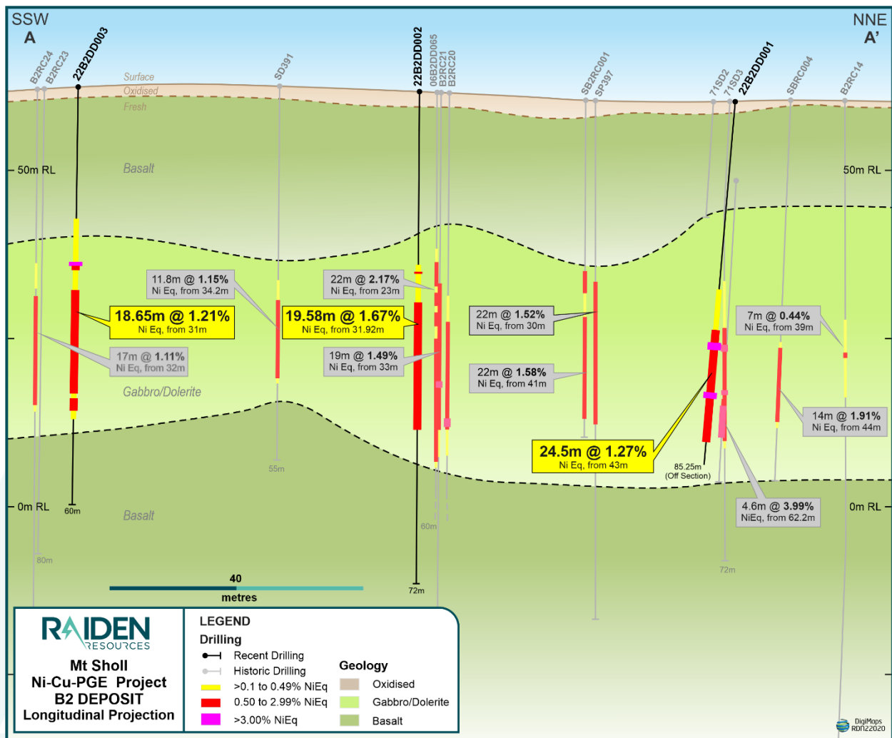
Figure 2: Long-section A-A' with recent holes and historical intercepts.
