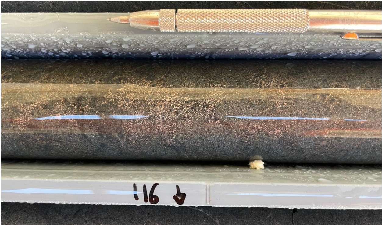
Figure 3: 22B1DD004 (approx. 115-116 metre interval – NQ core 47.6mm diameter). Strongly mineralised pyroxenite with fine-grained disseminated pyrrhotite mineralisation, with lesser chalcopyrite and pentlandite, within a 32.8 metre zone of sulphide mineralisation. 1
