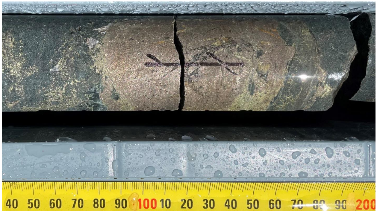
Figure 1: 22B1DD003 (101.3-101.4 metre interval – NQ core 47.6mm diameter). Mineralised dolerite with fine-grained massive pyrrhotite and chalcopyrite, with lesser pentlandite. Within a 22.2 metre zone of sulphide mineralisation. 1
