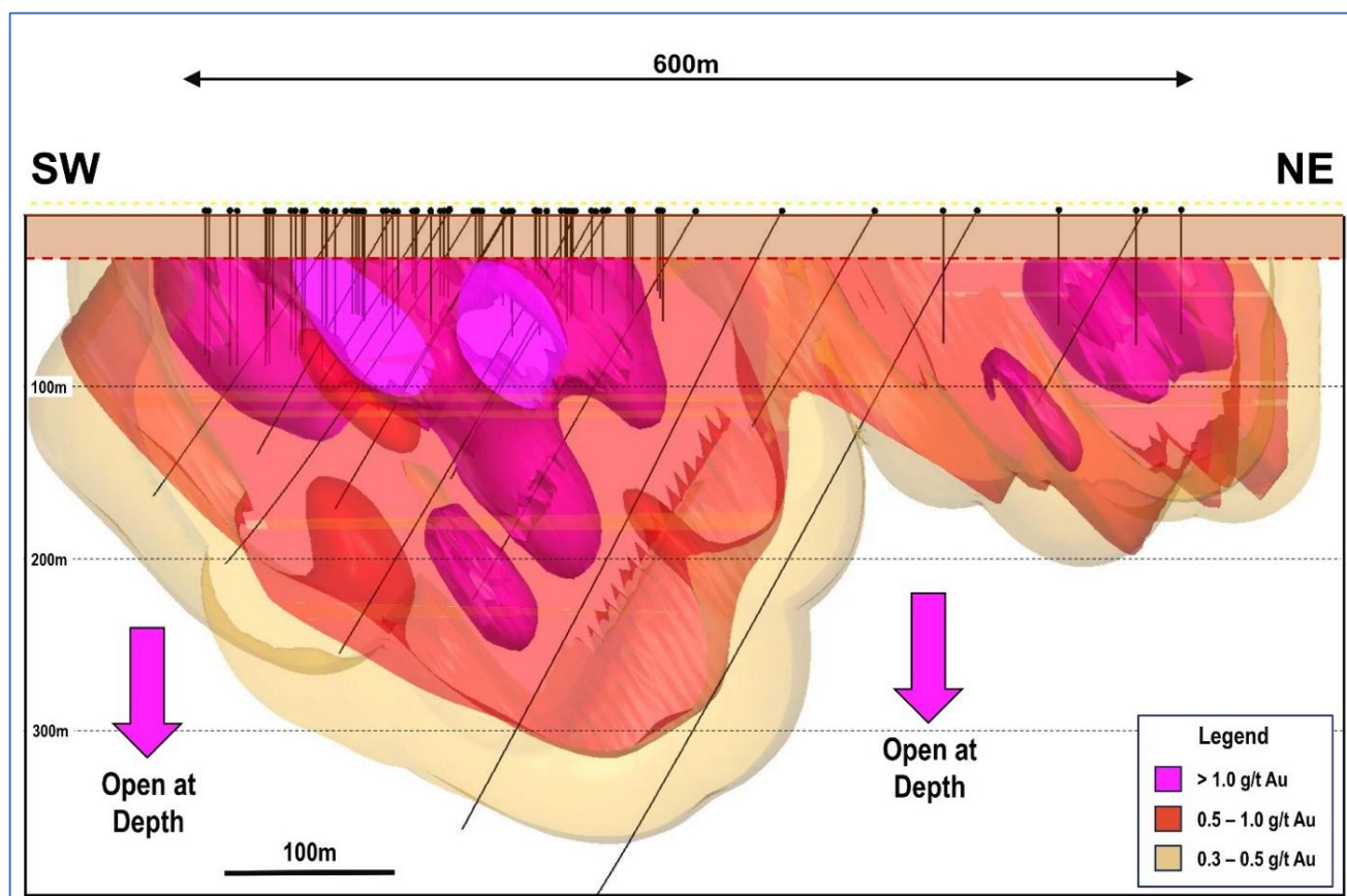
Figure 3: Cross-section of 3D Leapfrog software model. The interpretation illustrates gold grade shells, derived from all the significant intercepts reported to the ASX to April 2025. The Leapfrog model will be updated once all pending assays are received. The model is constrained via a 25m buffer to all the RGL/Oracle drill hole traces that have been drilled at Northern Zone since 2021. Refer to Figure 2 Drill collar plan for the location of the section line.
