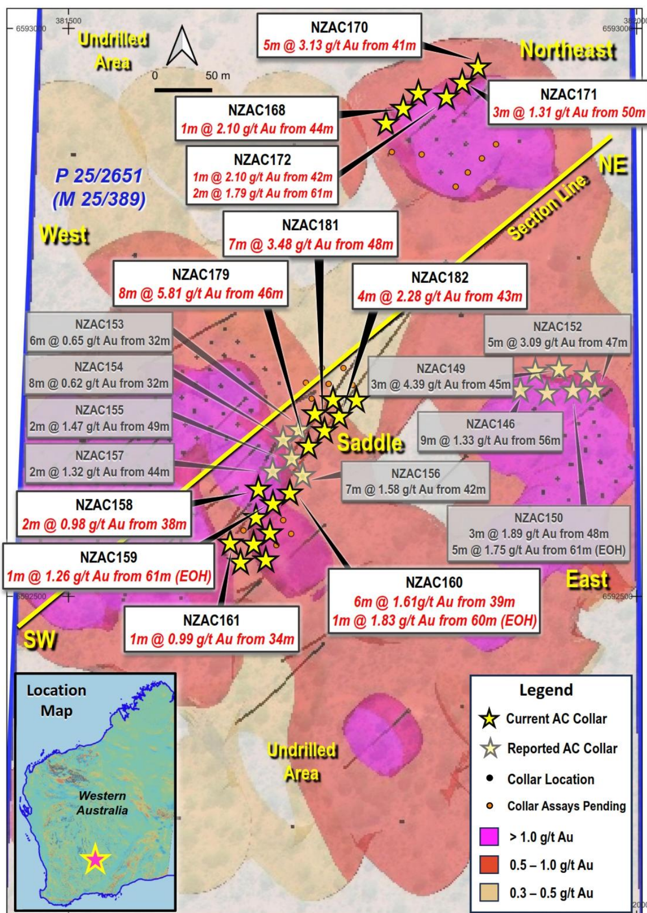
Figure 2: Drill collar plan and reported significant drill intercepts. Gold grade contours from all drilling results up to April 2025. Contours will be updated when all pending assays are received.
