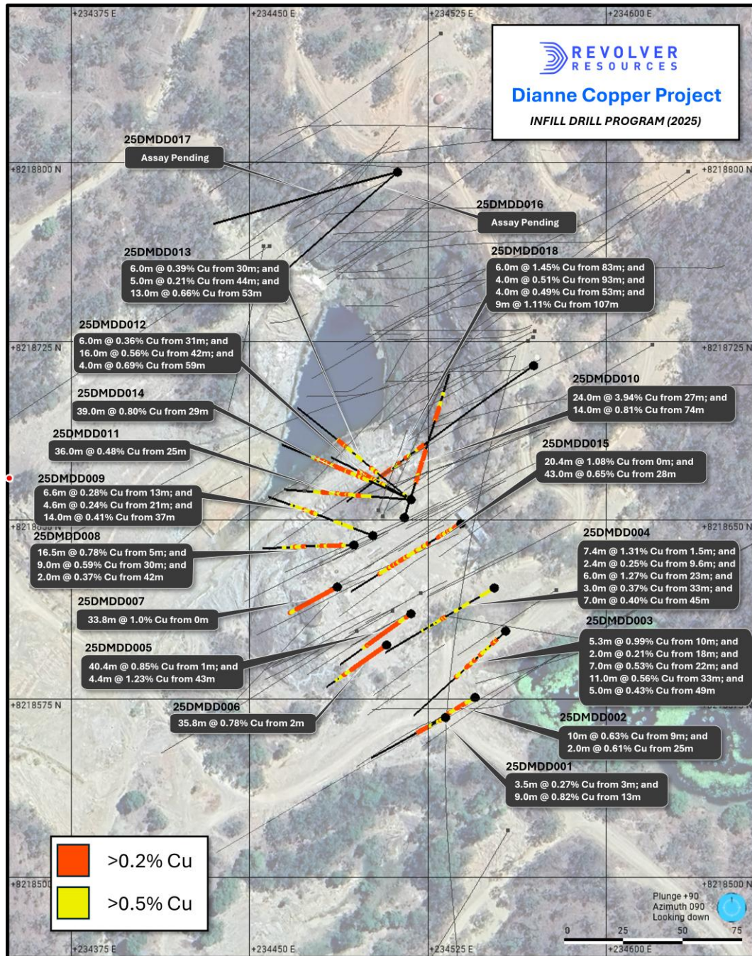
Figure 3: Drill program design – infill hole locations
