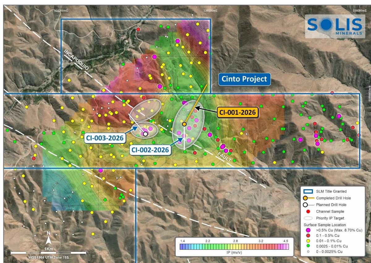
Figure 5: Cinto IP conductivity geophysical plot and historical geochemical sampling (grab and channel – Drill-holes CI-001-2026 through CI-003-2026 (with planned traces) illustrated
