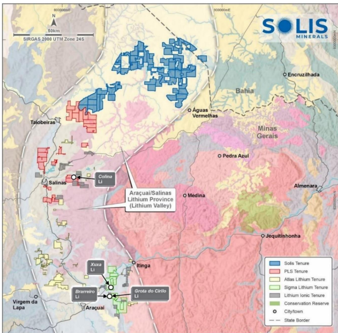
Figure 1: Araçuaí–Salinas Lithium Valley (illustrative). Regional spodumene operations (including Sigma Lithium) and exploration tenements held by Solis Minerals and other exploration companies
