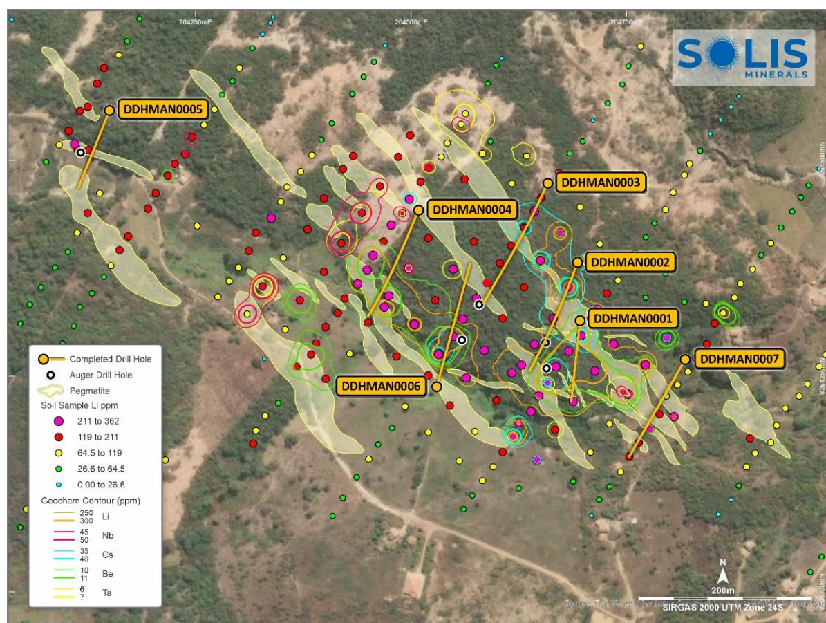
Figure 2: Mandacaru completed drill-hole collar locations and traces; over geochemistry results 4 , mapped pegmatites and interpreted geochemistry contours.
