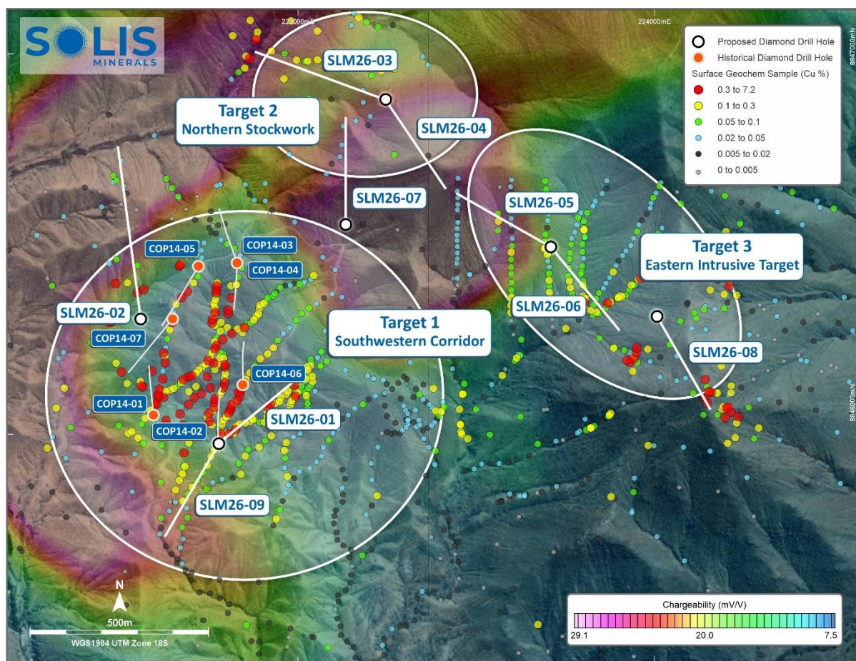
Figure 6: Cucho exploration area – target zones indicated with historical drillhole collars and traces, planned drill holes and traces, copper surface geochemistry and IP chargeability. A total of 34 drill holes have been permitted (not all shown) providing flexibility to adjust and scale-up the programme according to assay results.
