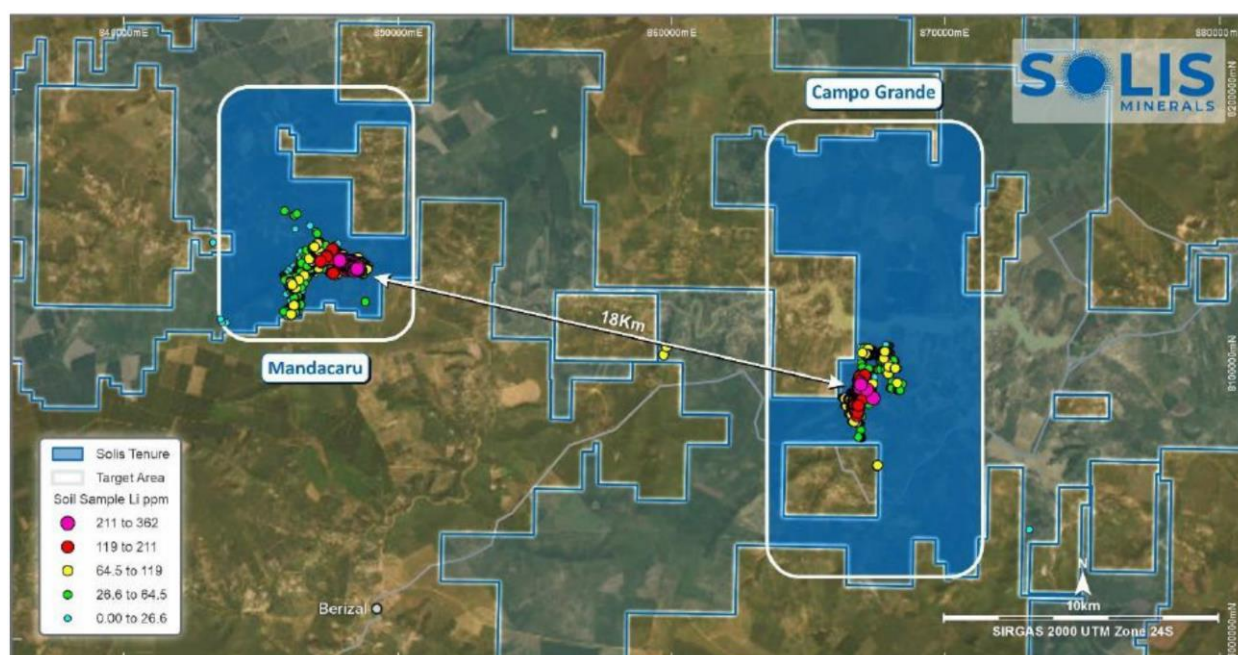
Figure 4: Brazil Lithium Project – Mandacaru and Campo Grande project areas located approximately 18 kilometres apart
