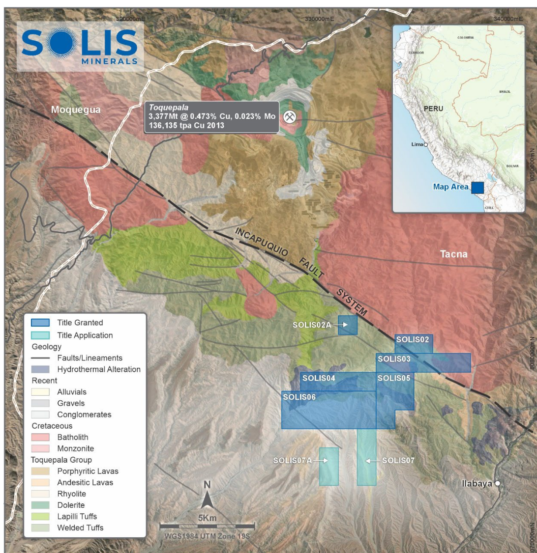
Figure 1: Cinto tenements, Incapuquio Fault System, and geology.
