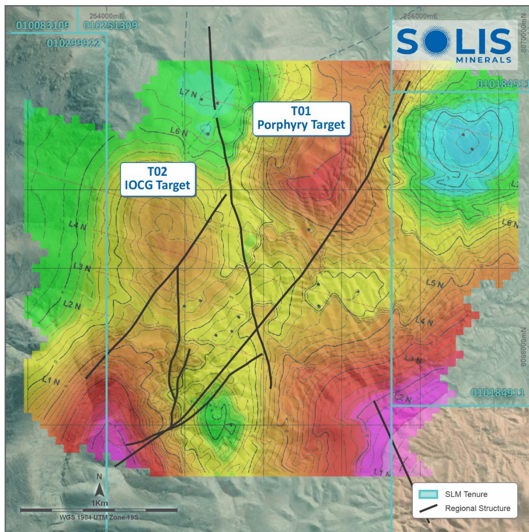
Figure 1; IP chargeability anomalies identified at Ilo Norte, Chanco al Palo project, Target 1 and Target 2 are coincident with Magnetic anomalies previously identified (see Figure 2, below).
