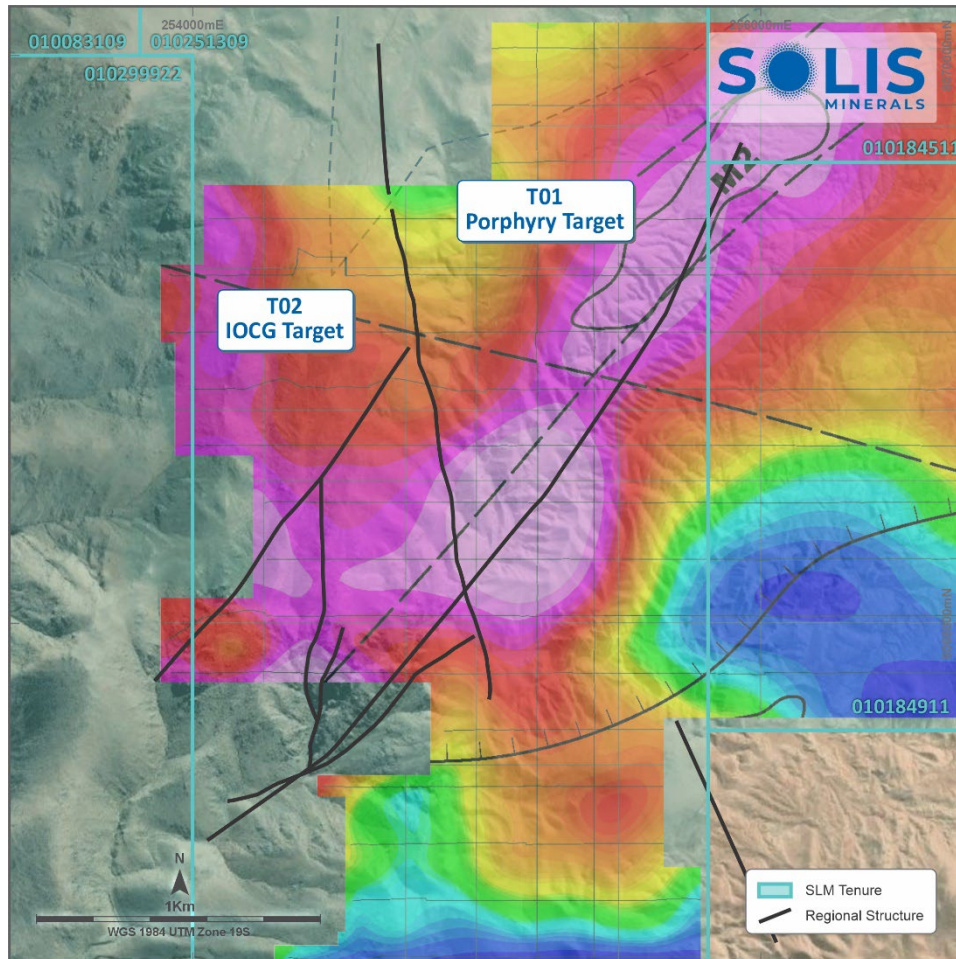
Figure 2; Drone magnetic RTP anomaly coincident with IP anomaly at Ilo Norte, Chancho al Palo project.
