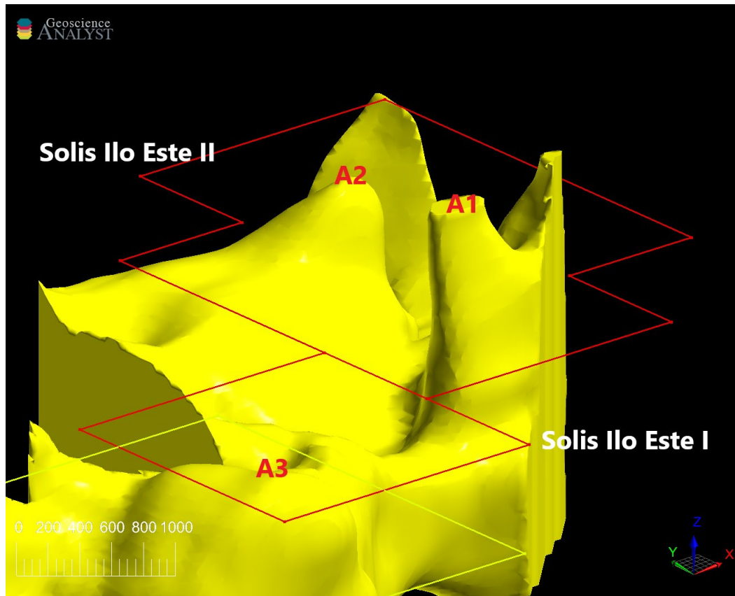
Figure 6; View of permits Solis Ilo Este I and II from the SW (minus 45 degrees) with induced magnetic anomalies shown as isosurfaces. A1 and A2 are anomalies in highly favourable structural settings indicating the potential presence of buried intrusives with associated magnetite. A3 is a subtler anomaly, probably more deeply buried than A1 or A2.
