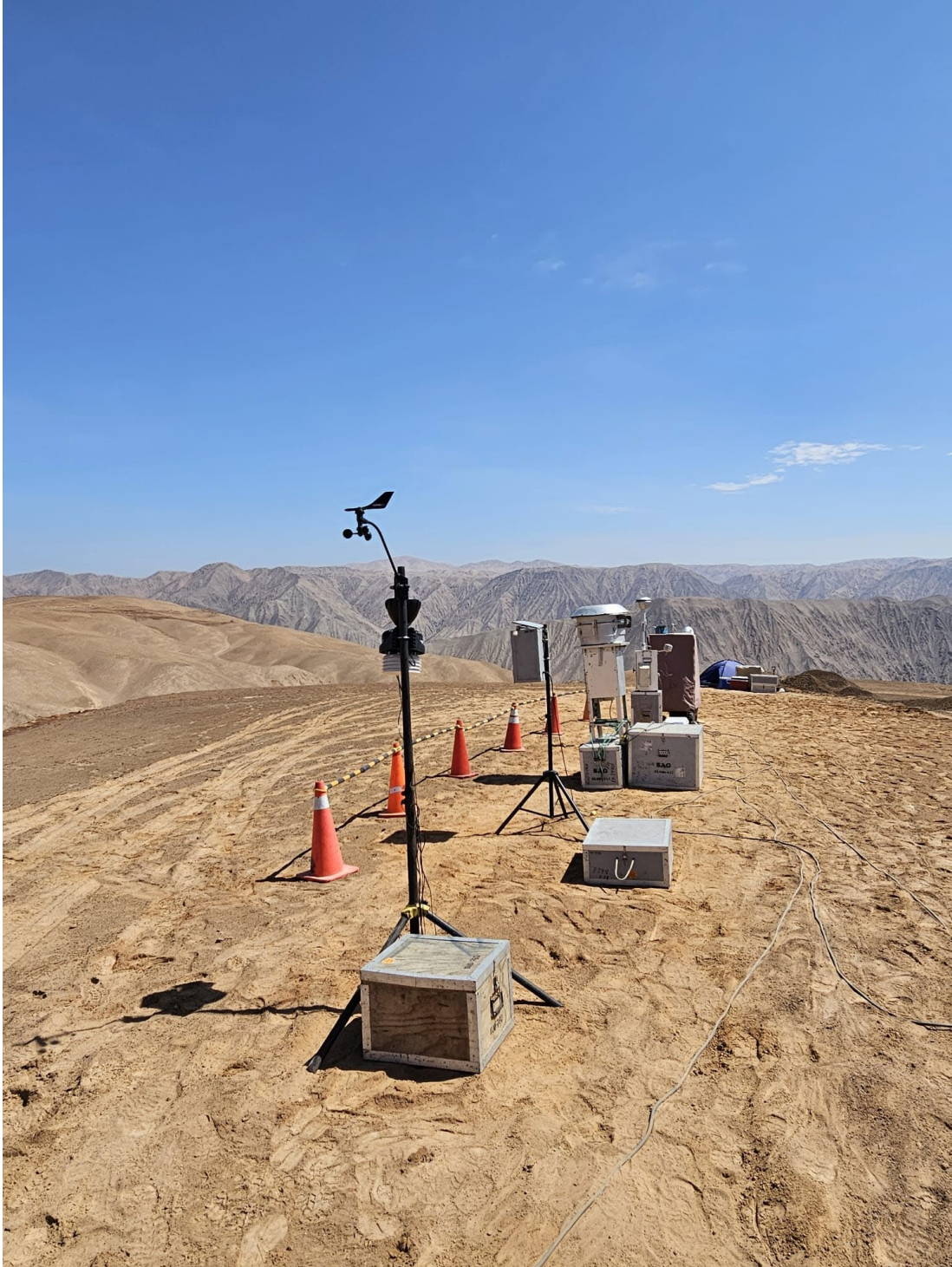
Figure 7; Environmental monitoring station at Ilo Este, April 2024. For drill permitting purposes, this station will remain operational for 24 hours a day for one month.
