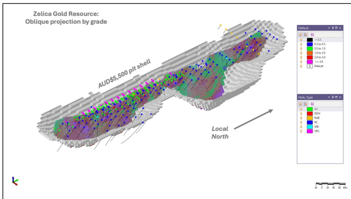
Figure 1: Zelica Gold Resource – Oblique Projection of resource defined by grade. Drill collars are represented by drill type
