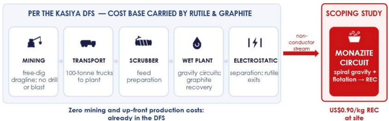
Figure 2: Kasiya's circuit to produce REC is added onto the DFS operation
