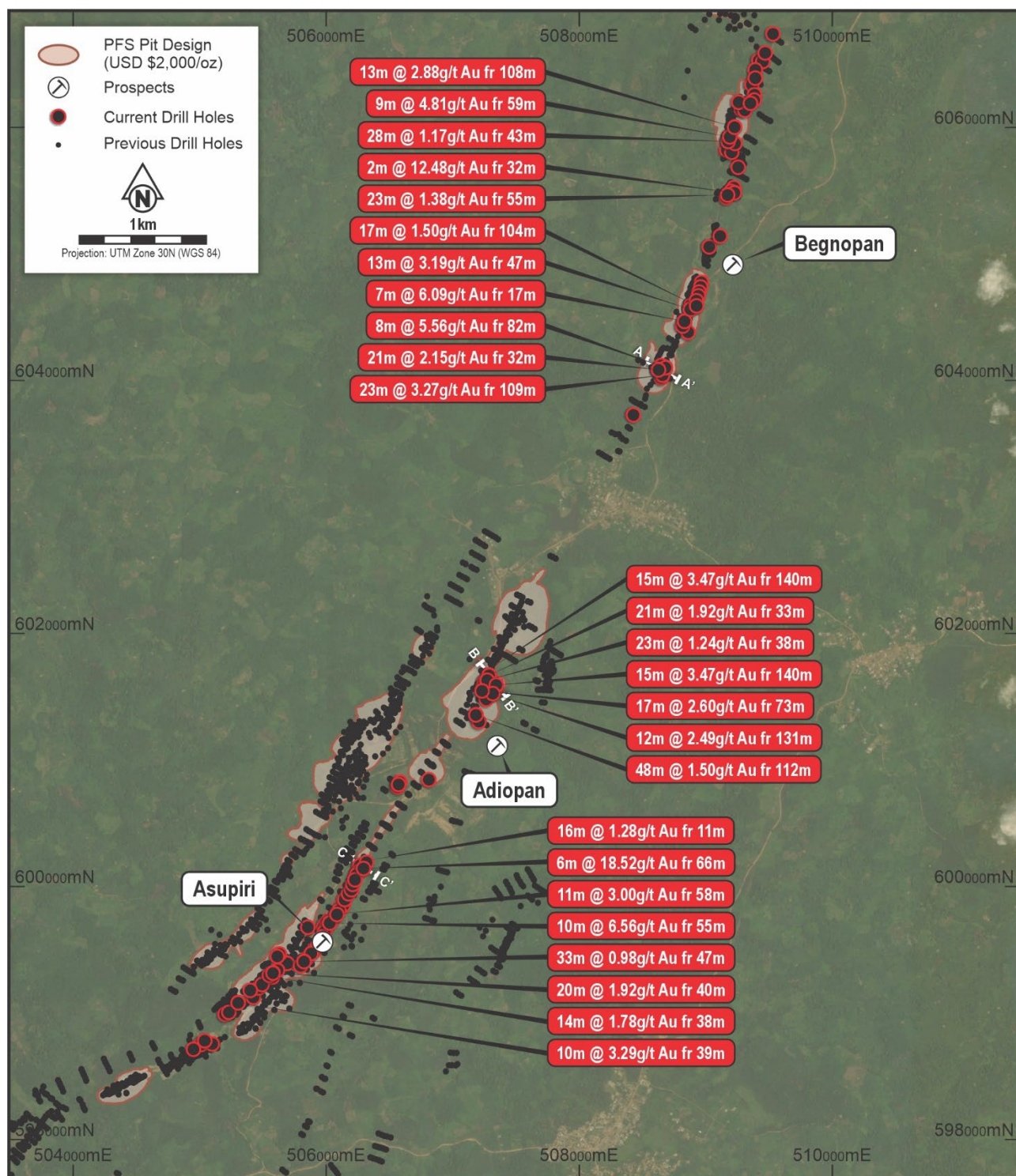
Figure Two | Drill Plan with Ore Reserve Open Pits
