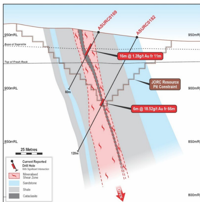
Figure Five | Asupiri Cross Section
