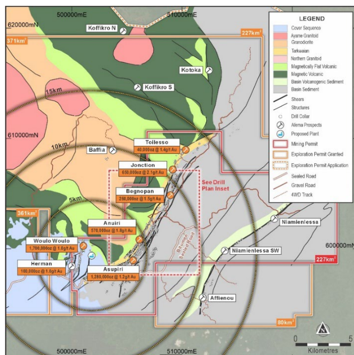
Figure One | Afema Mining Permit with Mineral Resources
