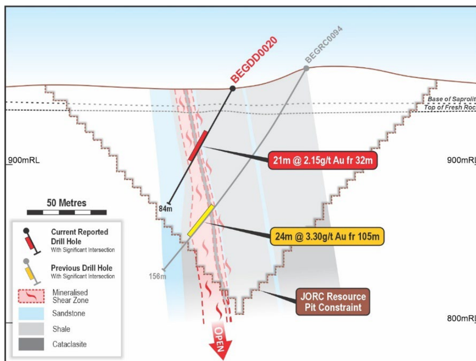
Figure Three | Begnopan Cross Section
