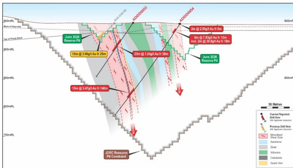
Figure Four | Adiopian Cross Section
