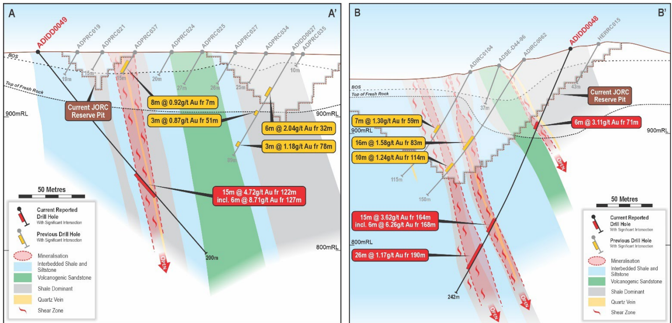
Figures Six and Seven | Adiopian Cross Section ADID0049 and ADID0048
