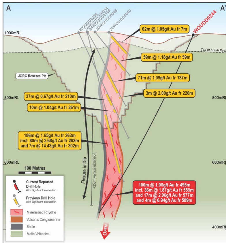
Figure Three | Woulo Woulo Cross Section WOUD0244
