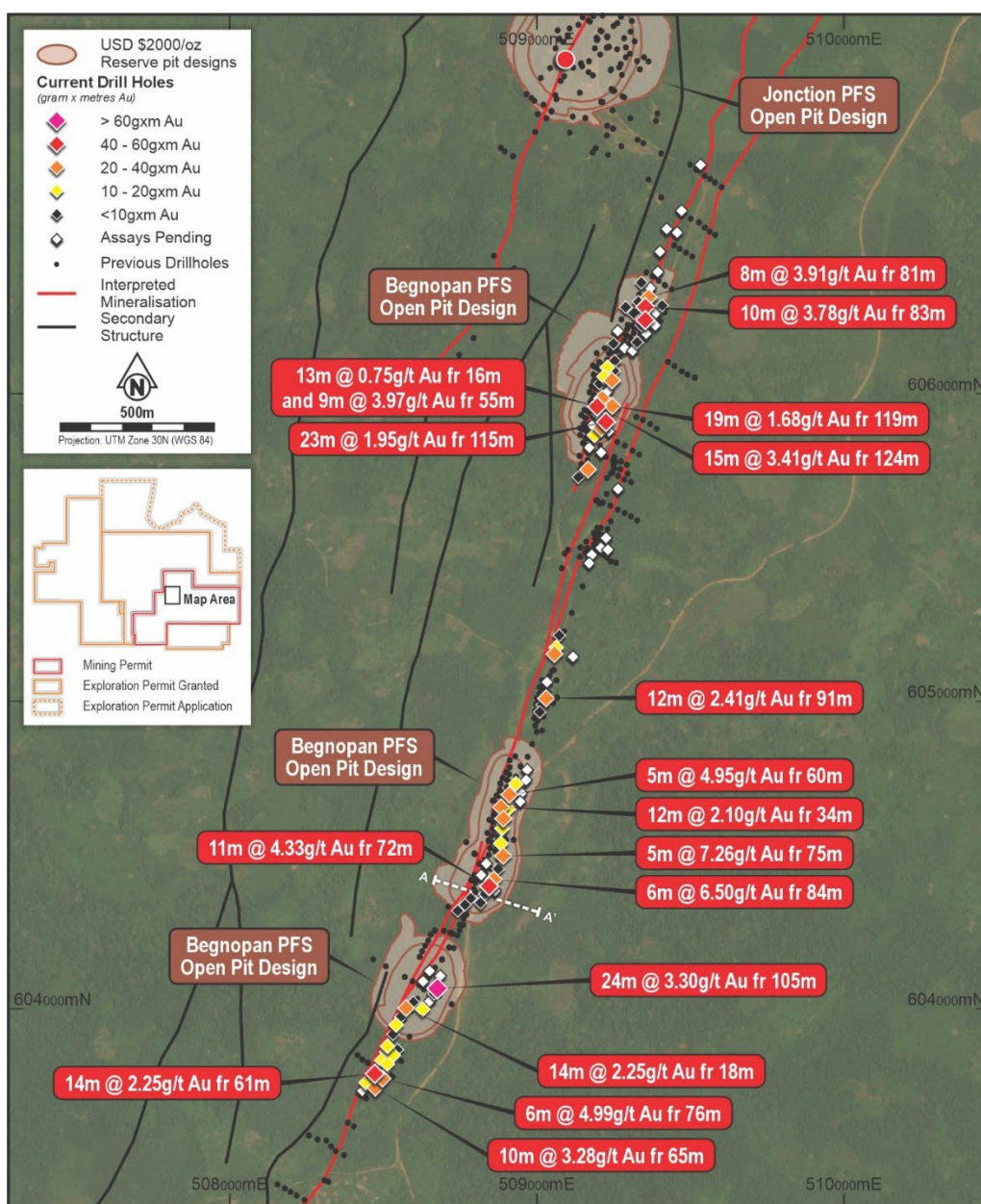
Figure Eight | Begnopan Drill Plan with JORC Ore Reserve Open Pits
