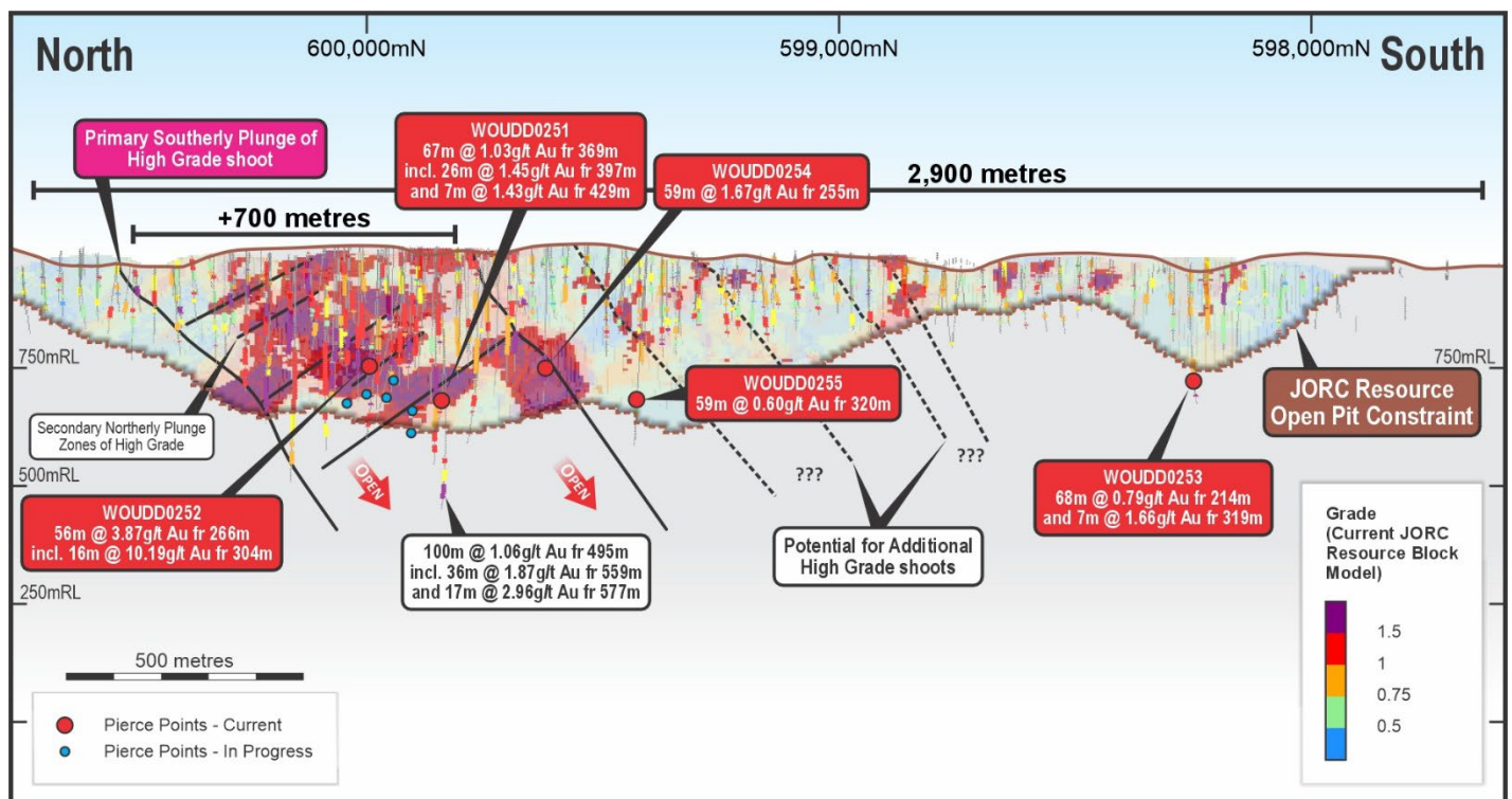
Figure Four | Woulo Woulo Long Section Block Model by Grade
