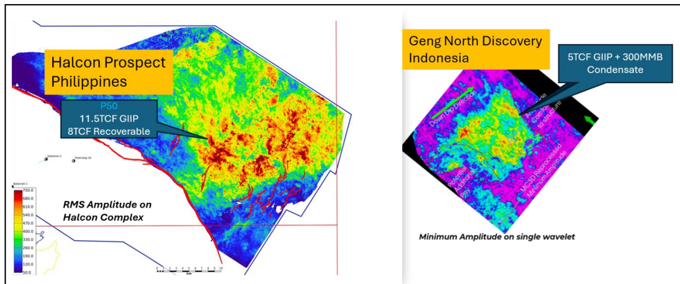
Figure 2 - Seismic amplitude comparisons between recent Geng North discovery made in Kutei basin of Indonesia by ENI and undrilled Halcon prospect in the Philippines. Two maps are at same scale. Image of Geng North is from public source data (Pei et al., 2025, Chasing the Geng North Play, enhancing direct hydrocarbon indicators through 3D seismic reprocessing in the Makassar Straits, 49th Annual IPA convention paper IPA25-G-177) (refer ASX release 3 September 2026).
