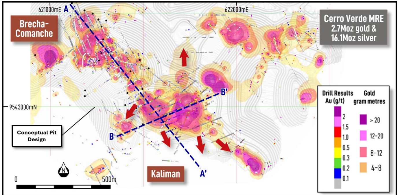
Figure 2. Plan View zooming in to display Brecha-Comanche and Kaliman targets within the Cerro Verde prospect, showing gold gram metre contours, conceptual pit design (US$3,500/oz gold), and drilling coloured by gold, with 2026 drilling marked by bold black collar markers. Note Kaliman mineralisation remains open in several directions.
