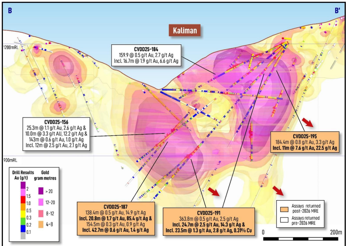
Figure 1. Kaliman Cross section looking northwest showing gold gram metre contours, drill traces coloured by gold and copper (red histogram), and latest significant drill intercepts highlighting wide zones of porphyry mineralisation and the presence of overprinting high grade epithermal mineralisation. Note that CVDD25-191 and CVDD25-195 assays have not previously been reported, while CVDD25-187 assays have been previously reported, but they were excluded from the 2026 MRE due to their arrival post assay cut-off date.
