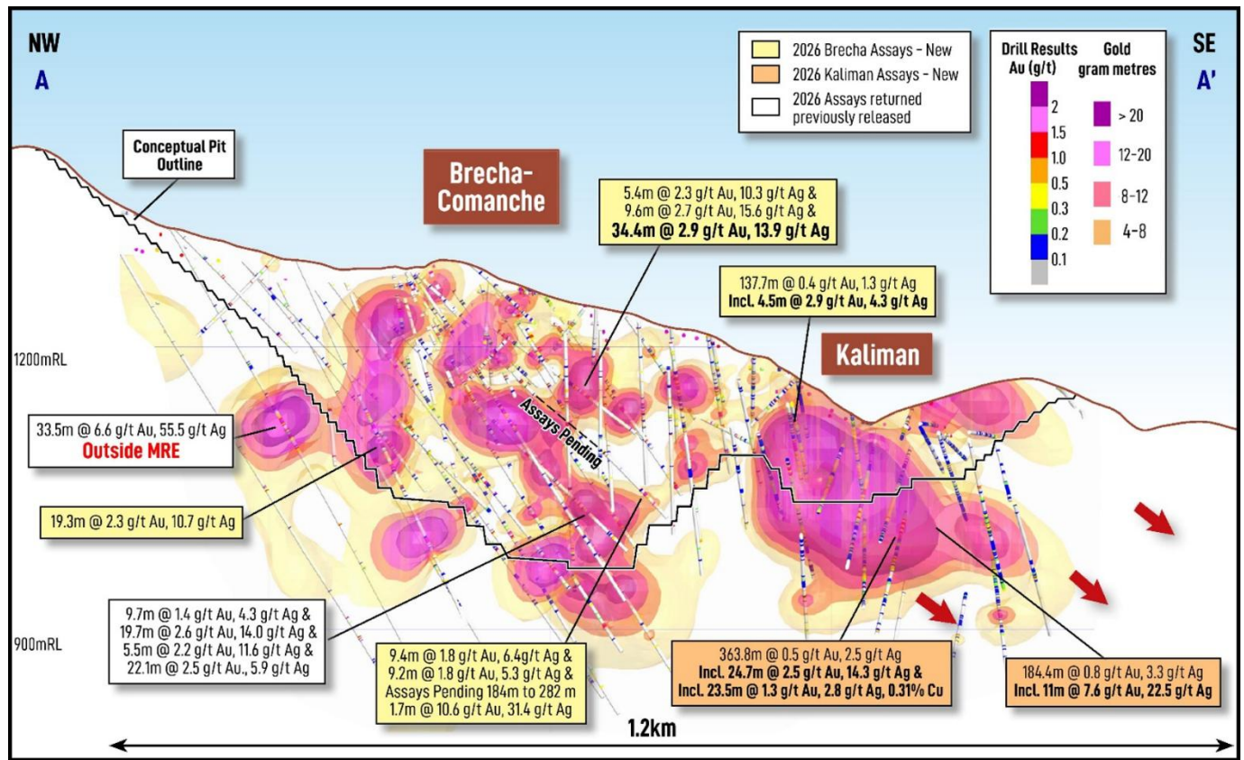
Figure 3. Long Section looking northeast (300m viewing window) displaying Brecha-Comanche and Kaliman targets, showing drill traces coloured by gold, gold gram metre contours, conceptual pit design (US$3,500/oz gold), and latest significant drill intercepts.
