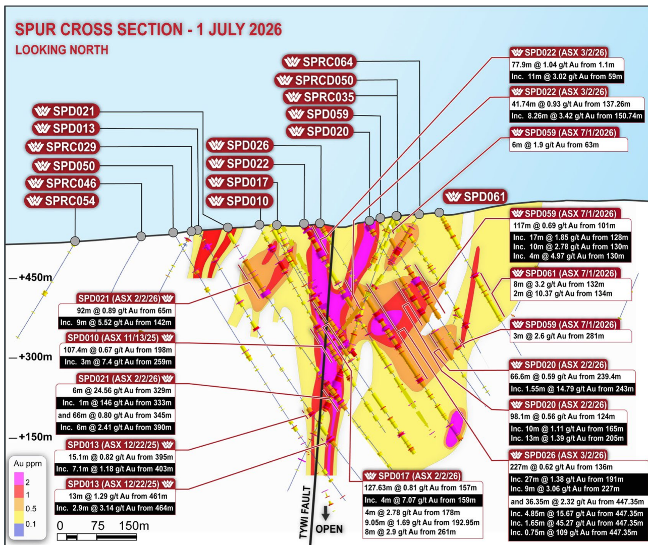
Figure 4: Spur Gold Zone Cross Section
