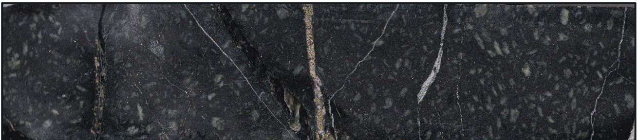
Figure 9: SPD022 69m 10.22 g/t Au. Monzonite with hematite dusted k-feldspar hosting pyrite-chalcopyrite-carbonate vein and pyrite veinlet
