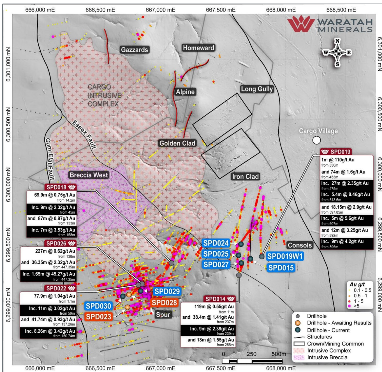
Figure 1: Spur Project, showing reported drilling
