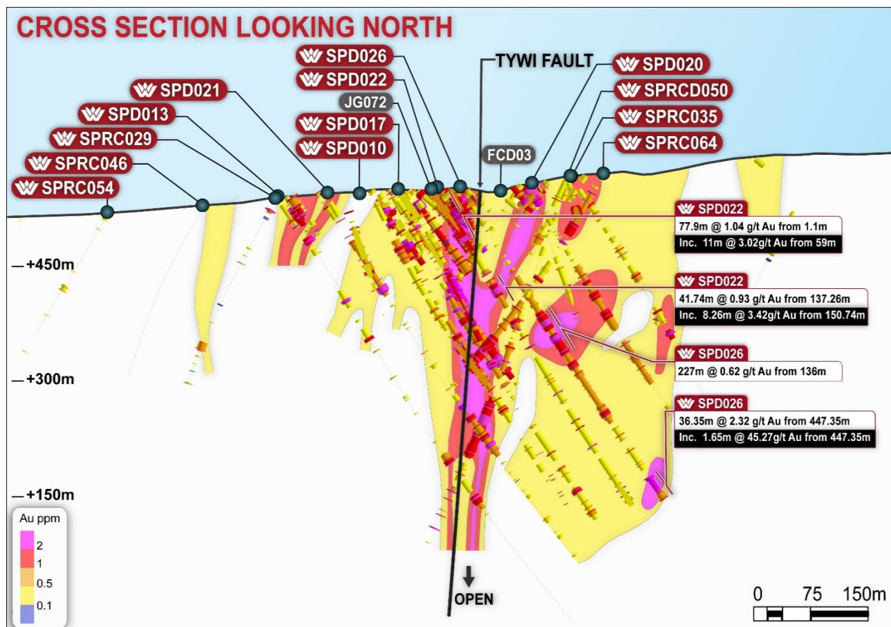
Figure 5: Spur Cross section showing SPD022 and SPD026
