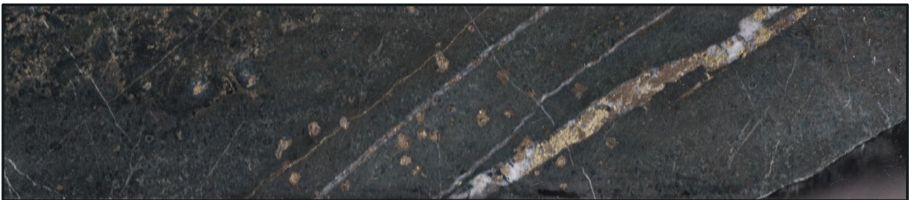
Figure 3: SPD019 515.5m 17.78 g/t Au. Basalt host rock with pyrite-chalcopyrite-quartz veins, pyrite veinlet and disseminated pyrite.
