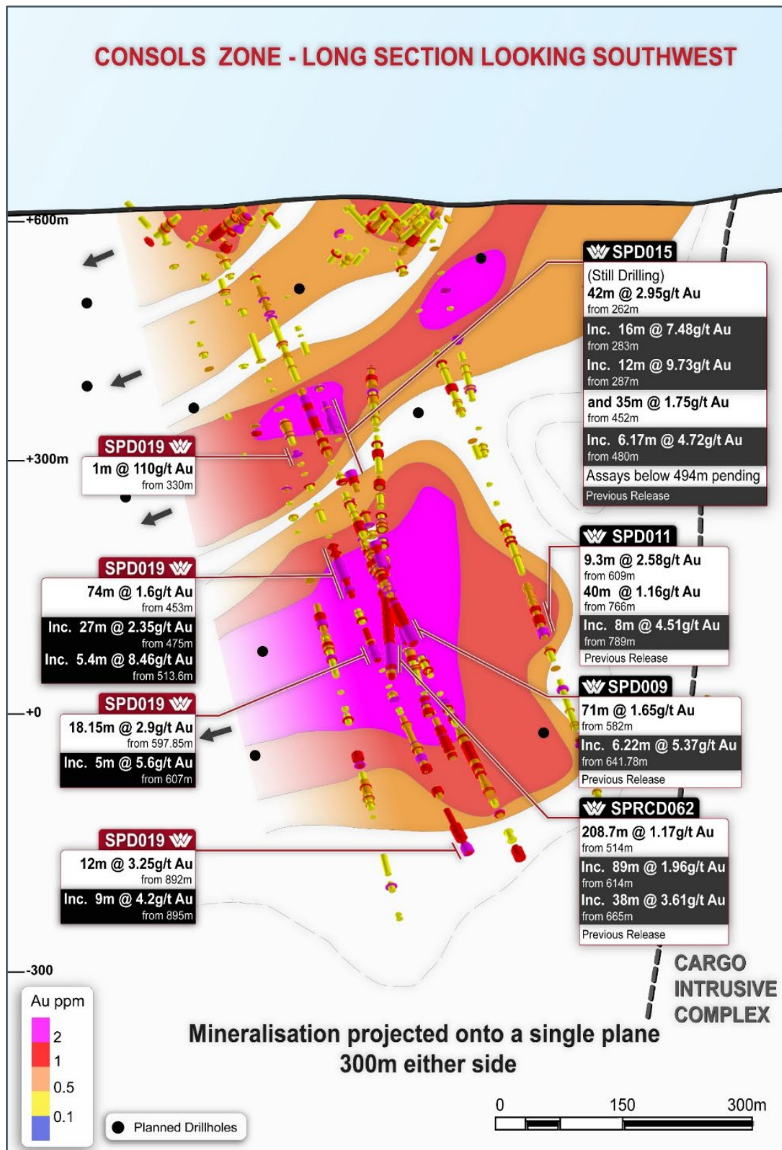
Figure 4: Consols, Long Section showing drilled mineralisation projected onto a single plane. Clipping window is 300m either side of the central plane. Drill hole SPD014 is too far behind the section and is obscured by SPD009, SPD015 and SPRCD062.
