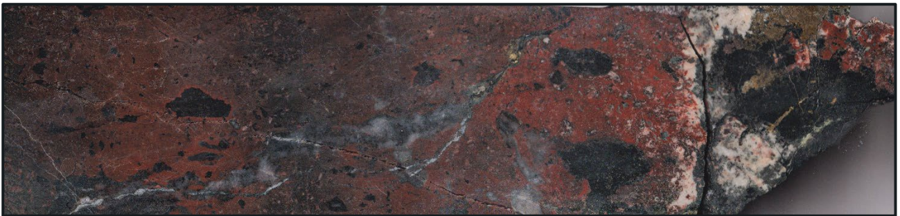
Figure 2: SPD019 330.4m 110 g/t Au. Fracture hosted Au in quartz altered andesite with later carbonate fault and hematite overprint.
