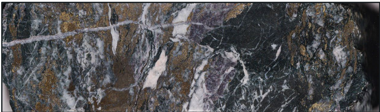
Figure 7: SPD026 447.8m 109 g/t Au. Quartz-carbonate-pyrite-chalcopryite shear zone. Image is 4.62 cm high
