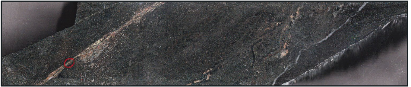
Figure 6: SPD018 169.3m, 6.77g/Au. Pyrite-quartz veinlet with potassic alteration in basalt. Image is 4.62cm high.
