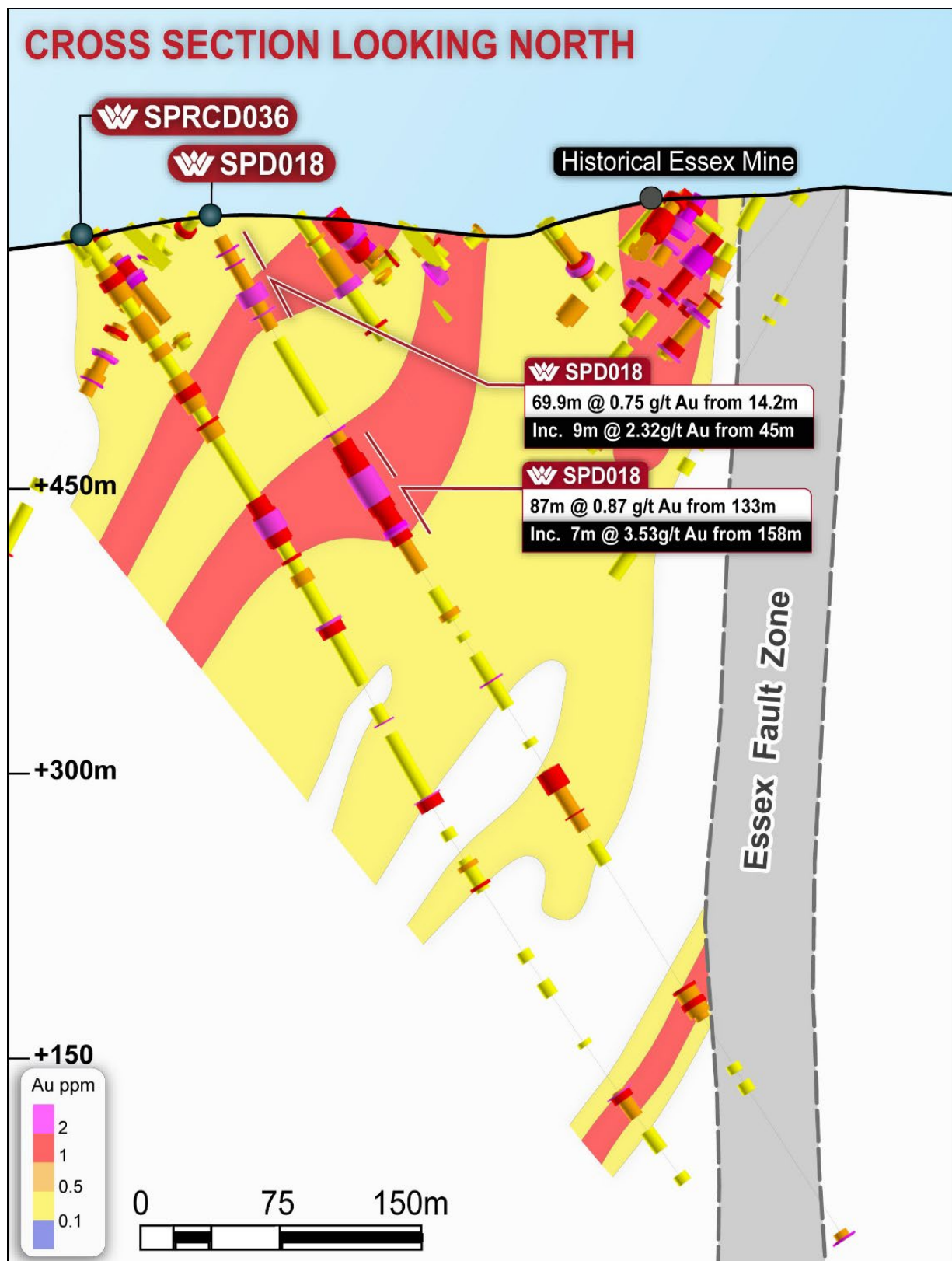
Figure 10: Spur Cross Section showing SPD018
