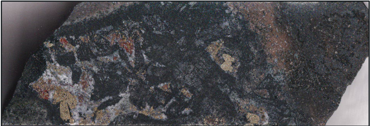
Figure 8: SPD026 208.8m 10.69 g/t Au. Intermediate sulphidation breccia with quartz-carbonate-pyrite-magnetite infill and calc-potassic alteration hosted in andeiste. Image is 4.62cm high.
