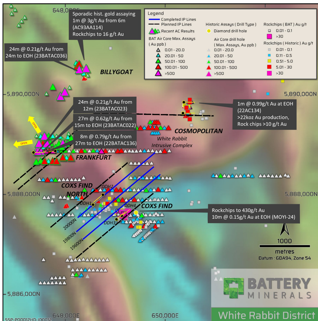
Figure 1: White Rabbit District, showing main prospects, drilling coverage, rockchip geochem, IP coverage over RTP magnetics
