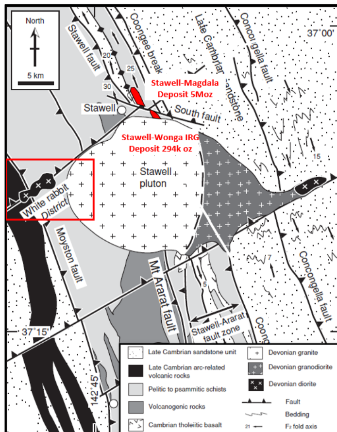
Figure 4: Geological summary map of Stawell Region, modified from Miller and Wilson 2004
