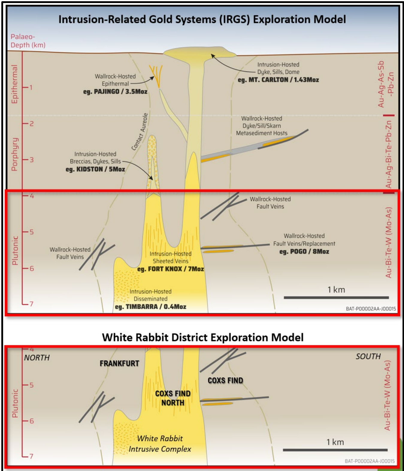
Figure 5: Schematic exploration model for varying styles of mineralisation within an Intrusion-Related Gold System (IRGS) and within the White Rabbit District
