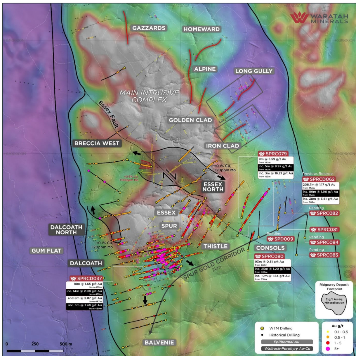
Figure 7: Spur Project, Main Intrusive Complex Targets, Spurr Gold Corridor and other epithermal and porphyry targets, drilling coverage, major surface geochemical trends over RTP magnetics
