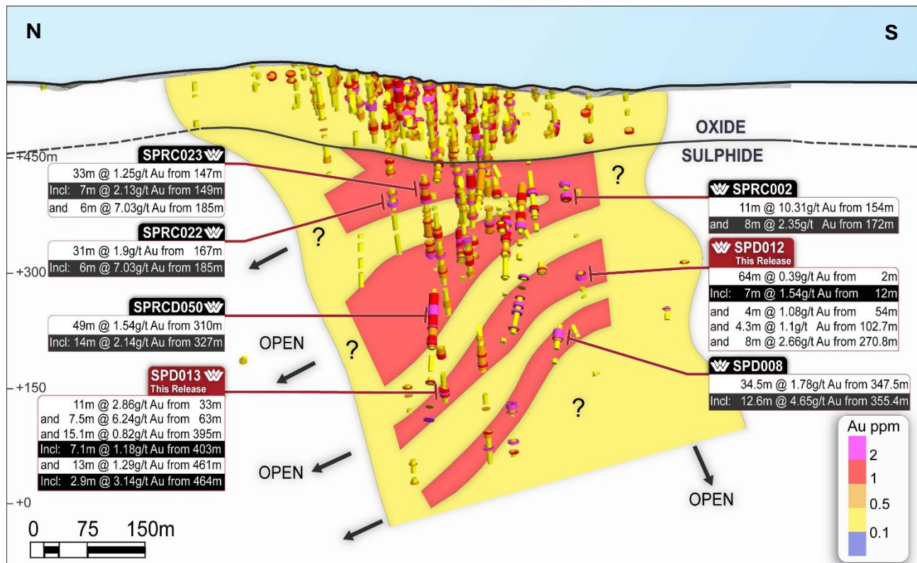
Figure 4: Spur Project, Long Section
