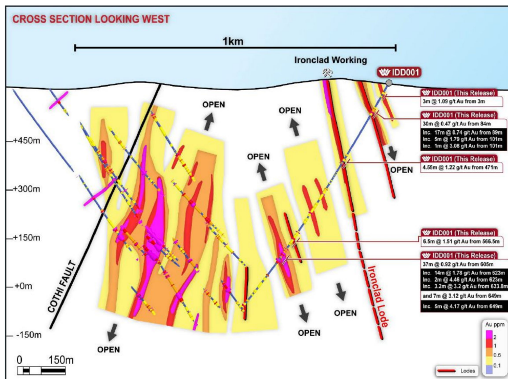
Figure 7: Spur Project, Section through Consols to Ironclad showing drill hole IDD001, intercepts and growth potential between Consols and Ironclad
