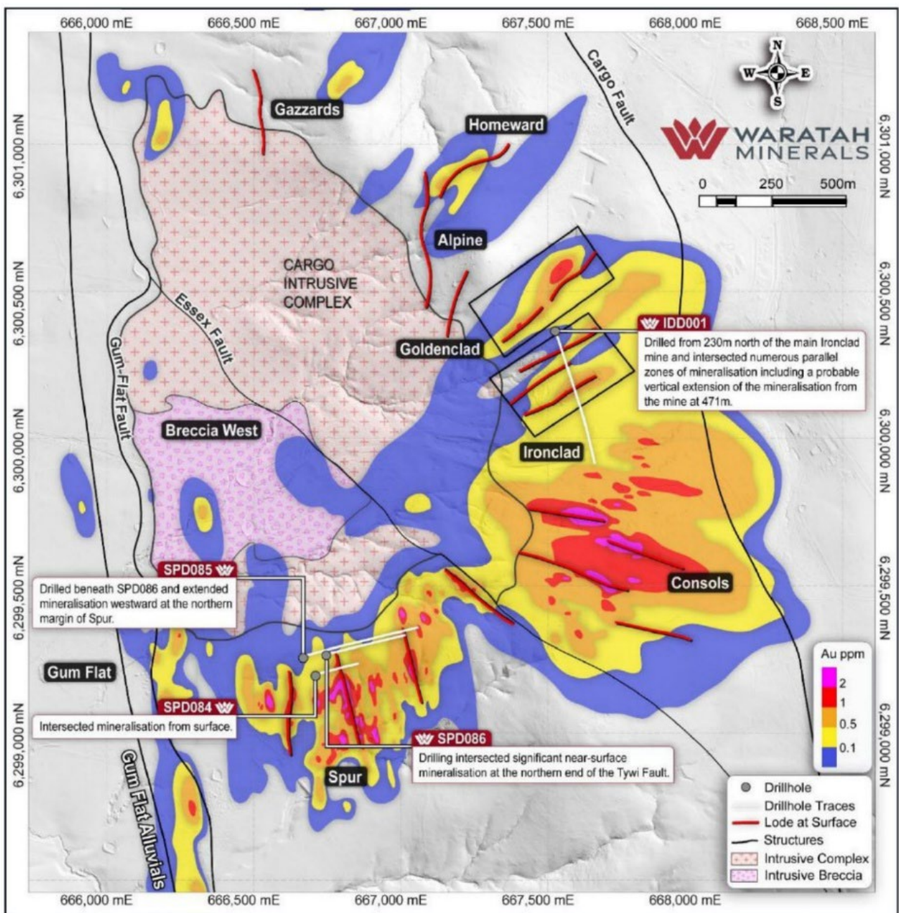
Figure 5: Spur Project, showing reported drilling results and growth potential. Gold mineralisation contours projected to surface
