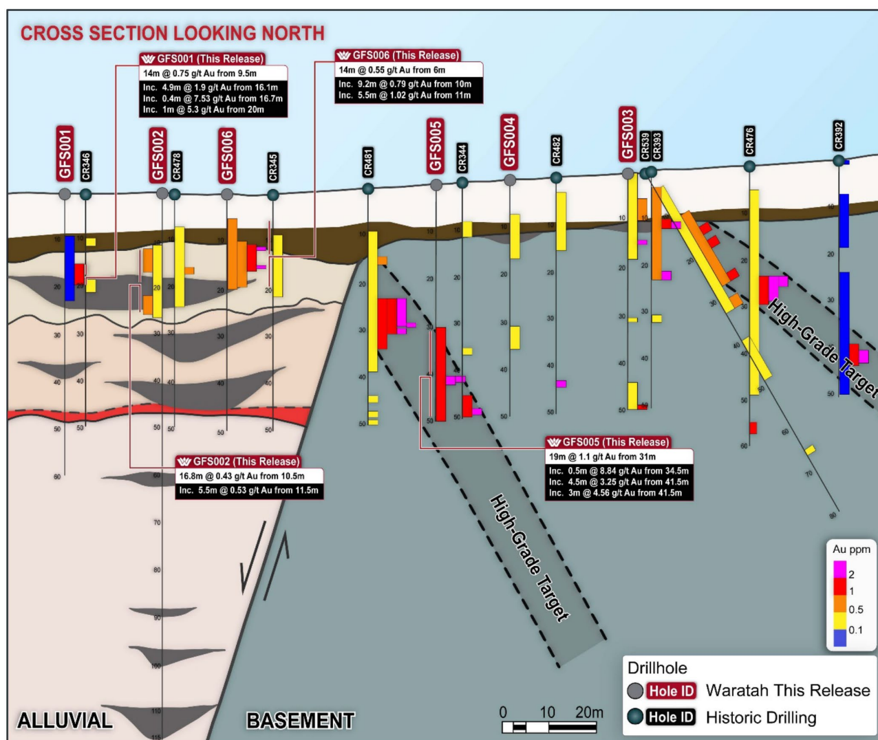
Figure 9: Spur Project, Gum Flat drill section showing alluvial and eluvial gold zones
