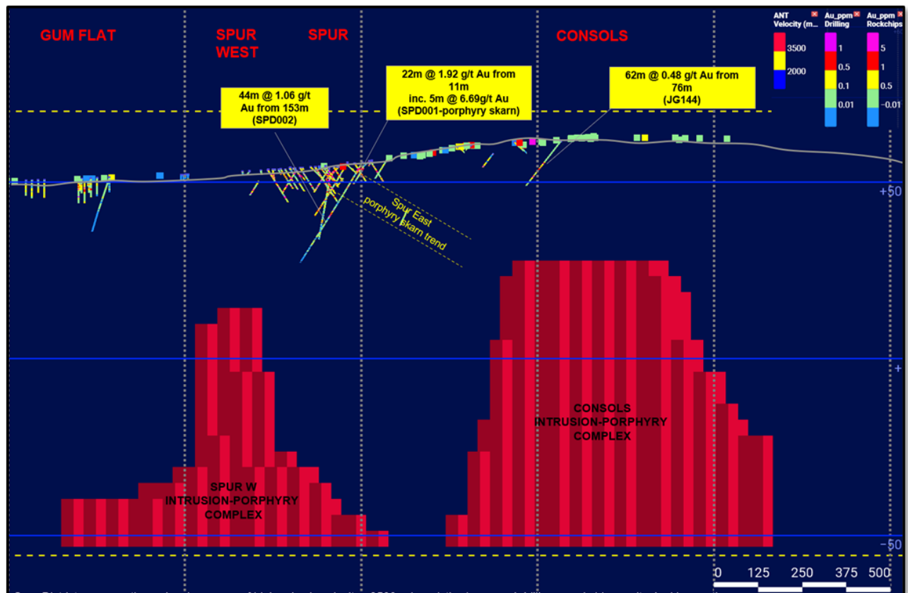
Figure 3: Spur District cross section, showing zones of high seismic velocity >3500m/s, looking north
