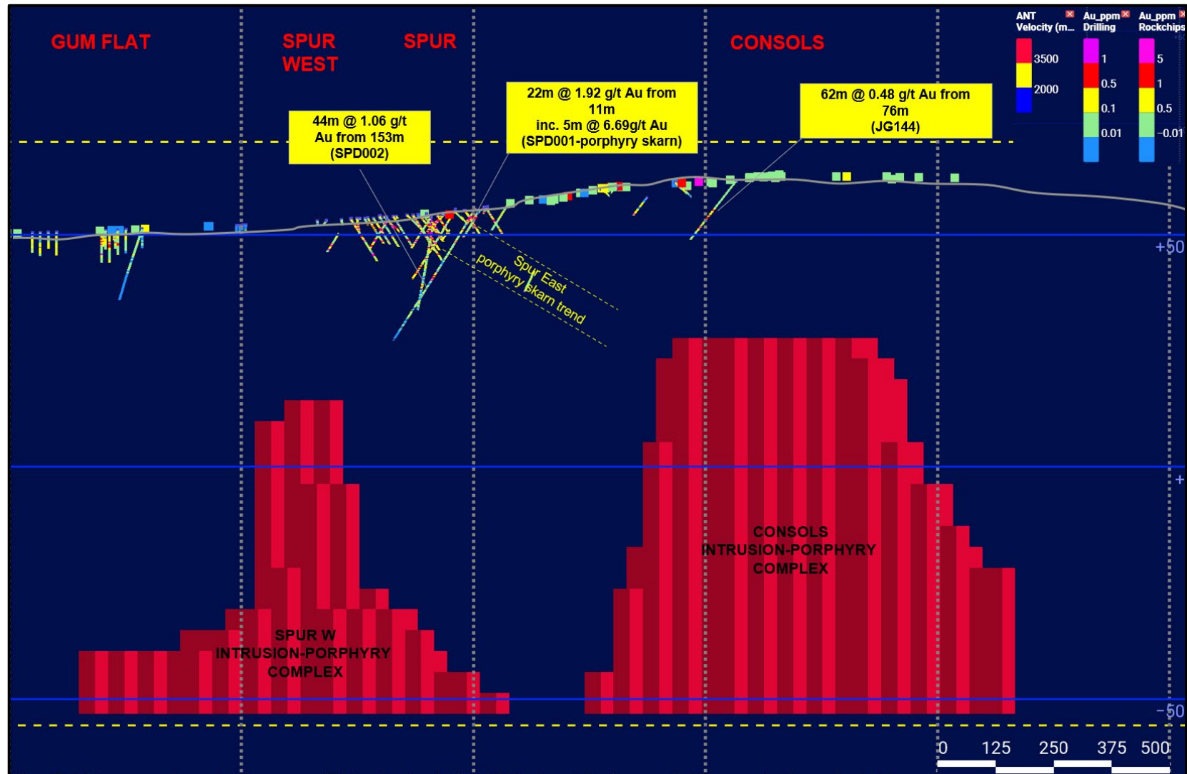
Figure 4: Spur District cross section, showing zones of high seismic velocity >3500m/s, looking north
