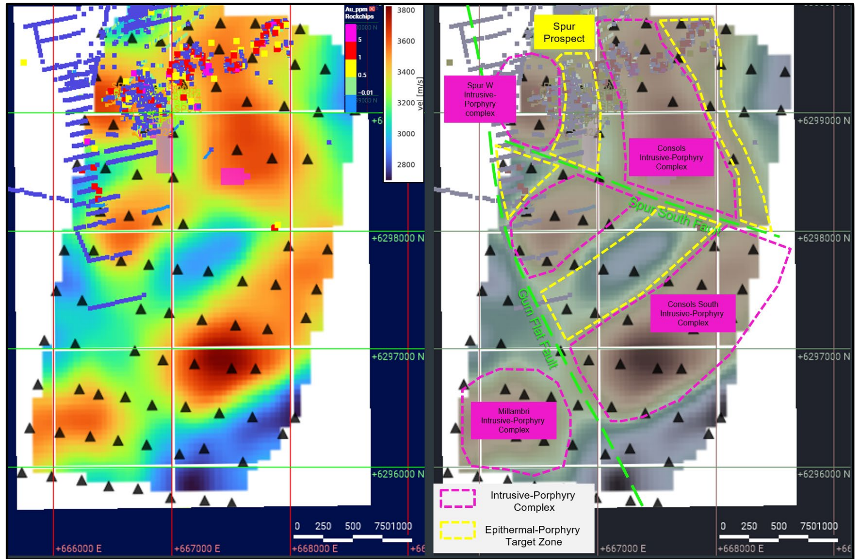
Figure 3: ANT shear velocity model, depth inversion at 500m depth, providing definition of discrete high velocity zones, interpreted as new and extensions of large intrusion-porphyry complexes
