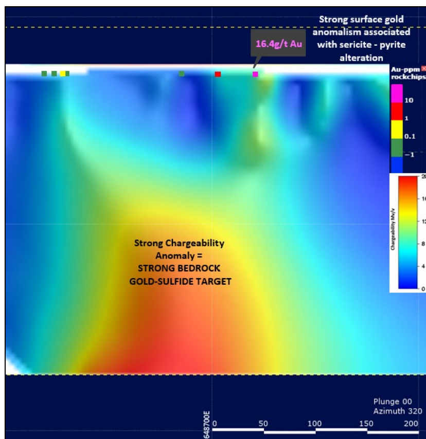
Figure 1: IP Chargeability Inversion, Section 20000N, showing strong IP chargeability anomaly beneath high grade gold-sulphide mineralisation in rockchips (historical data in ASX BAT 14 October 2021) (200m window), see Appendix 1 for sections and inversions
