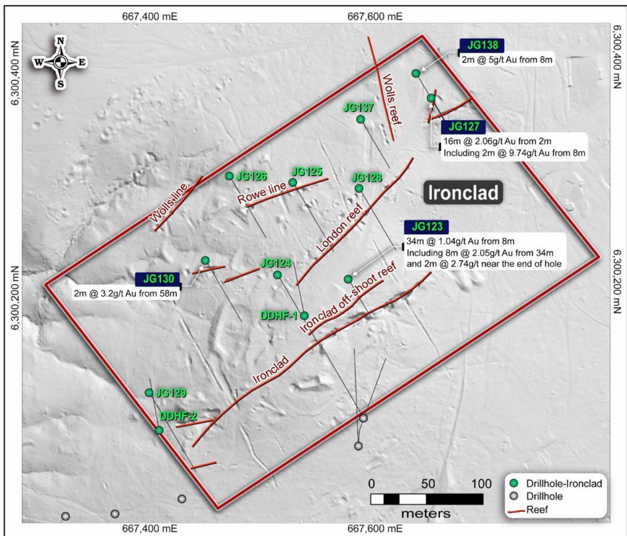
Figure 2: Ironclad Mining Lease with mapped lodes and historic drilling by Golden Cross Golden Cross Resources (1997), Ironclad GL5828 Annual Report: https://digs.geoscience.nsw.gov.au/api/download/c28fef663d3d21aa6d02cd90a4ac1bfc/Thirty_third_annual_exploration_report_G_R00002858_2025-10-29.pdf
